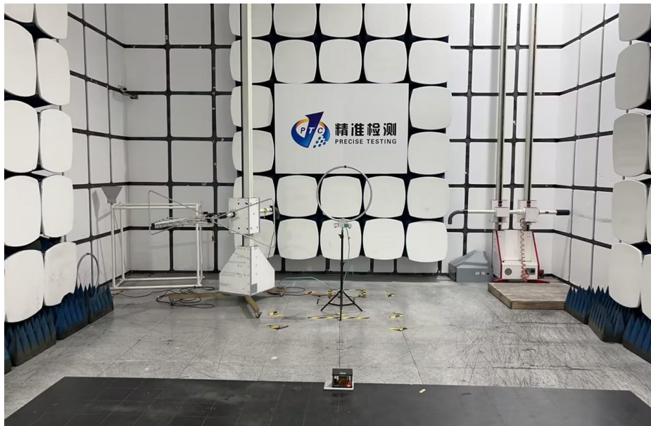
Radiated Spurious Emissions 9KHz-30MHz
