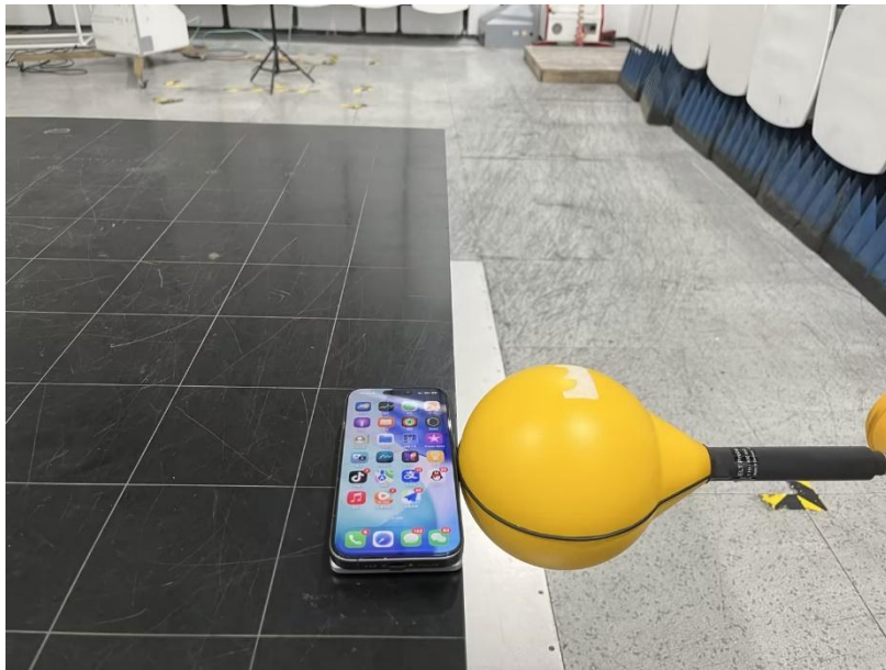
Electric Field Strength Top Test setup:
