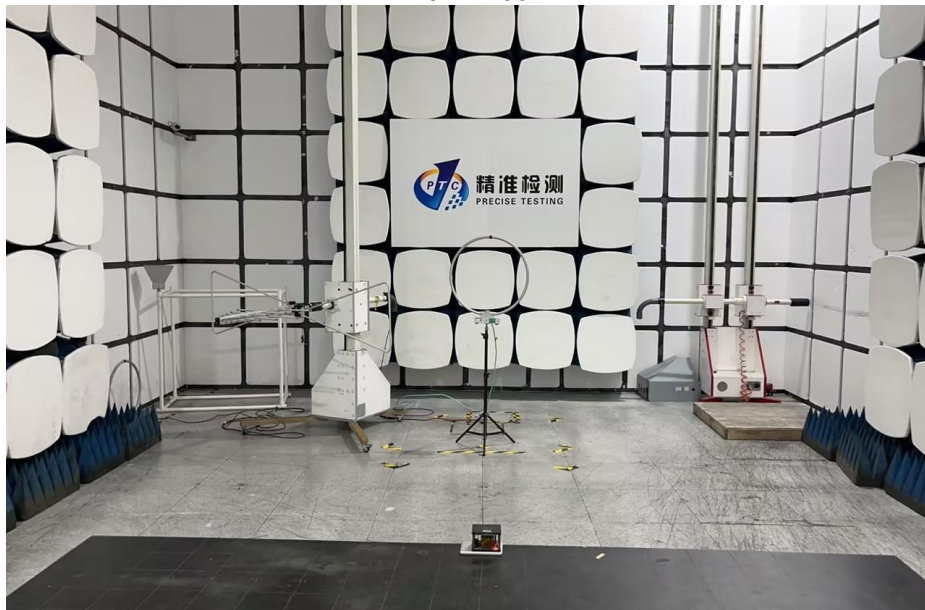
Radiated Spurious Emissions From 9KHz-30MHz
