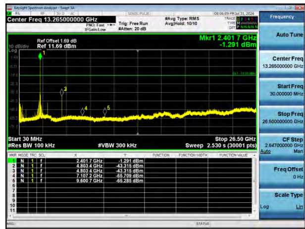
Spurious Emissions
