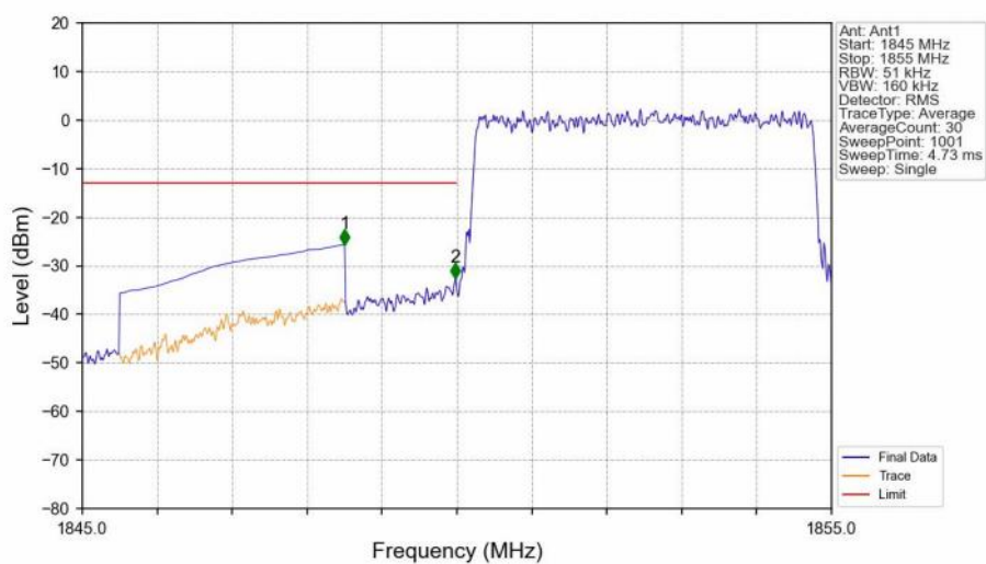
Band2_5MHz_16QAM_LCH_1852.5MHz_RB_25_0_NTNV
