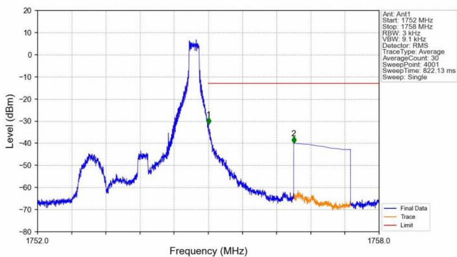
Band4_1.4MHz_QPSK_HCH_1754.3MHz_RB_1_5_NTNV
