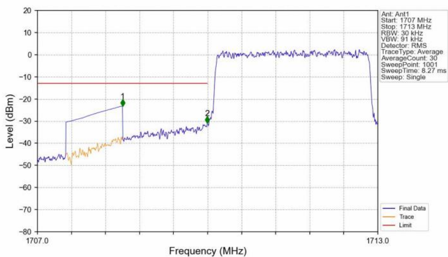
Band4_3MHz_16QAM_LCH_1711.5MHz_RB_15_0_NTNV
