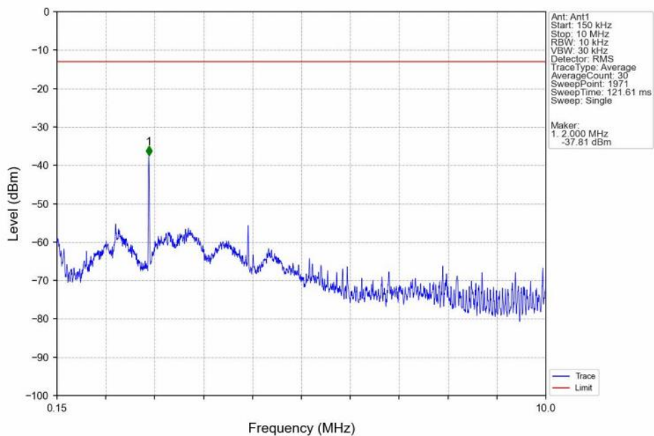
Band4_10MHz_16QAM_MCH_1732.5MHz_RB_1_0_NTNV
