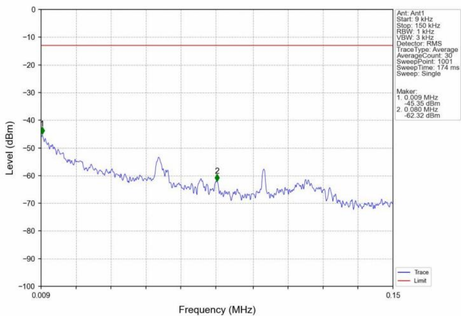
Band4_20MHz_16QAM_MCH_1732.5MHz_RB_1_0_NTNV
