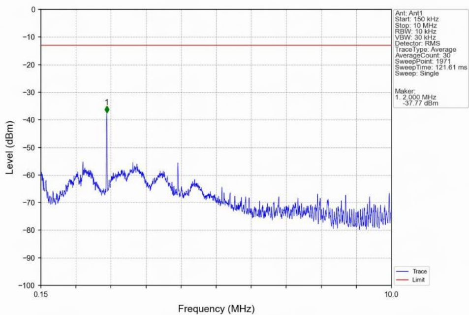
Band4_10MHz_16QAM_HCH_1750MHz_RB_1_0_NTNV
