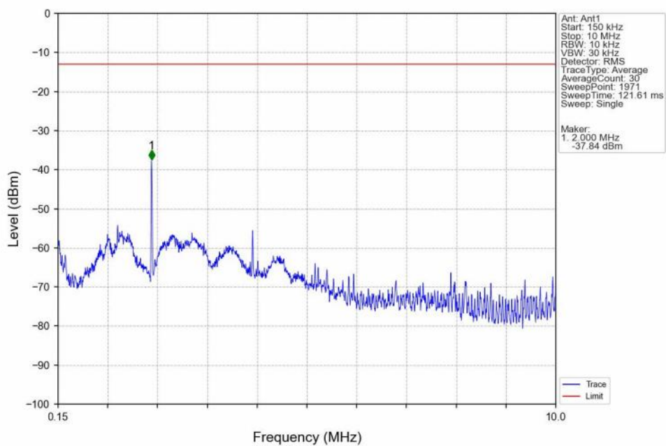
Band4_15MHz_16QAM_HCH_1747.5MHz_RB_1_0_NTNV
