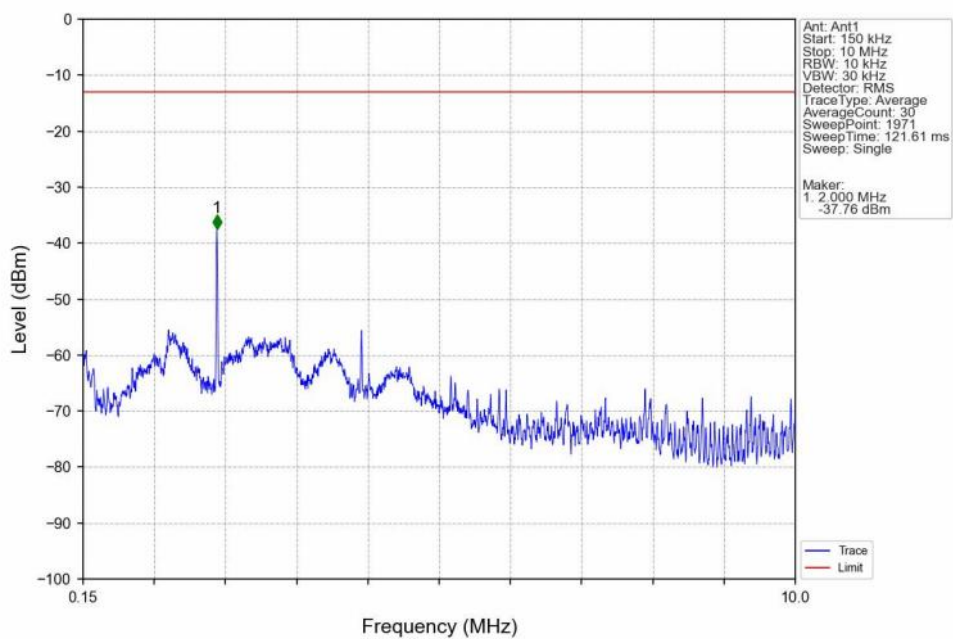
Band4_10MHz_16QAM_LCH_1715MHz_RB_1_0_NTNV
