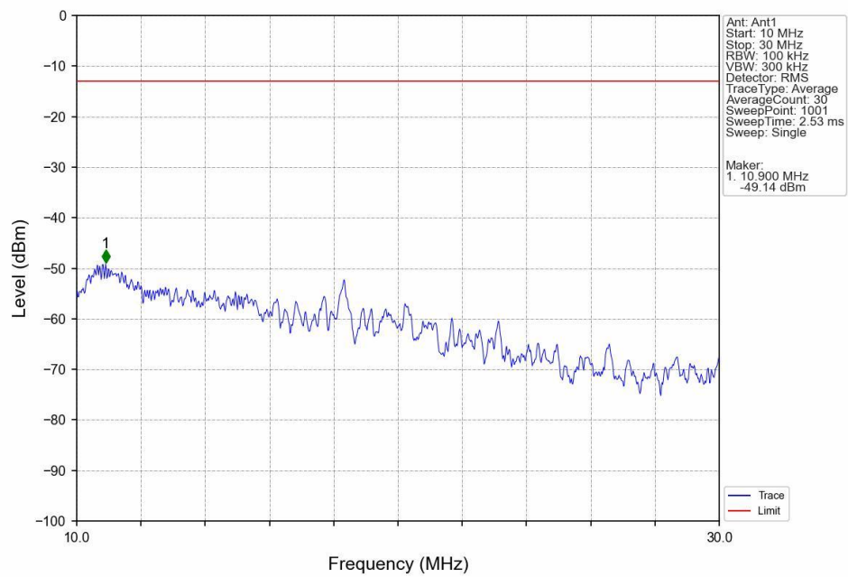
Band2_HSDPA_MCH_1880MHz_Subtest 1_NTNV
