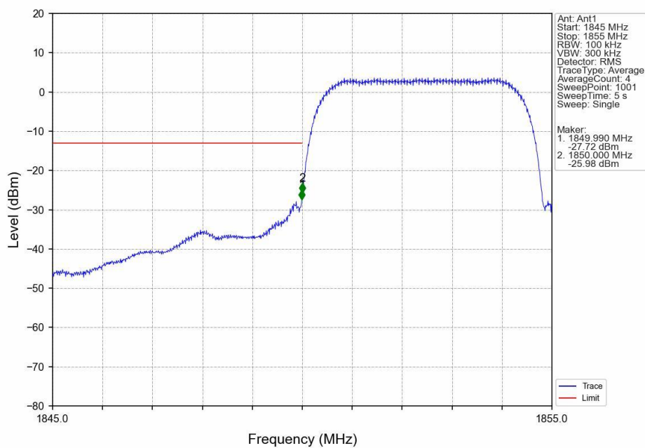
Band2_HSDPA_LCH_1852.4MHz_Subtest 1_NTNV
