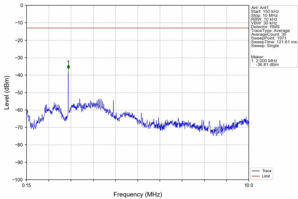
Band5_HSDPA_HCH_846.6MHz_Subtest 1_NTNV
