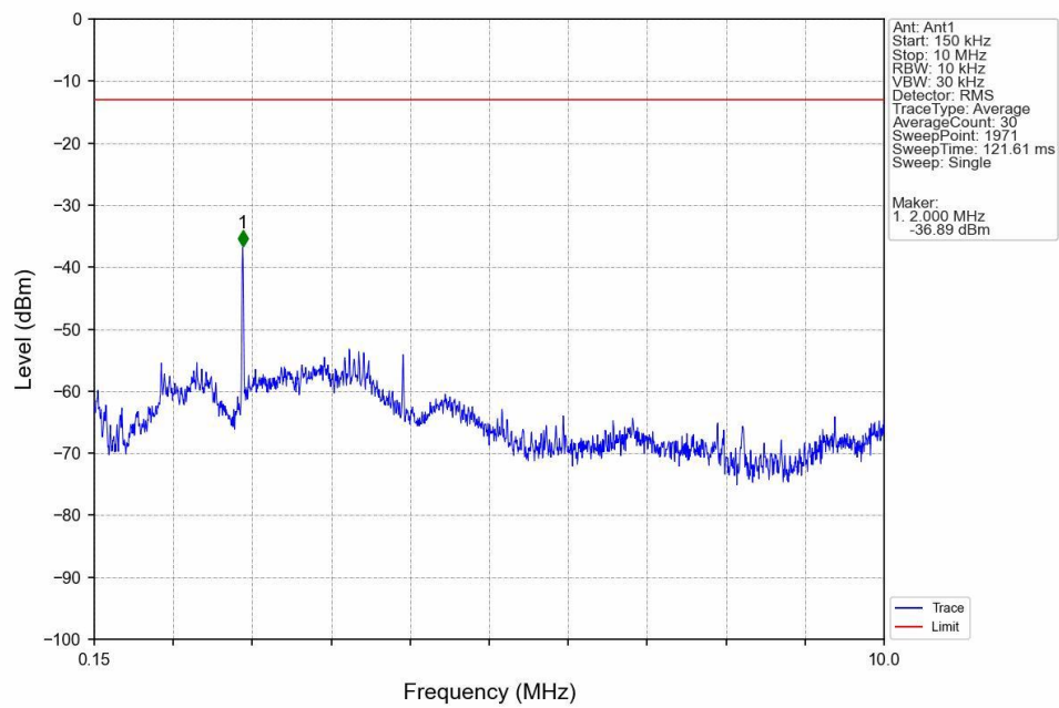
Band5_HSUPA_HCH_846.6MHz_Subtest 1_NTNV
