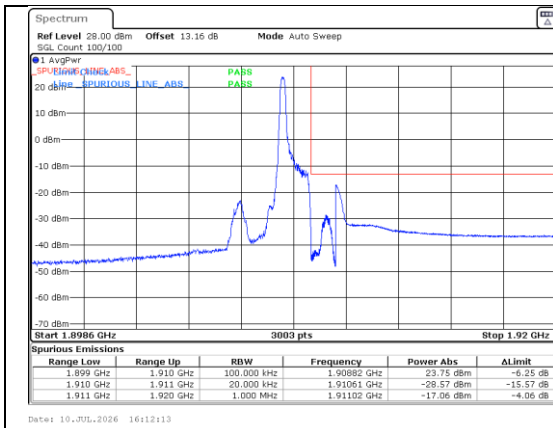
Band 2 1.4MHz/1909.3/High QPSK 1@0
