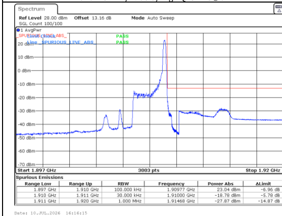
Band 2 3MHz/1908.5/High 16QAM 1@14
