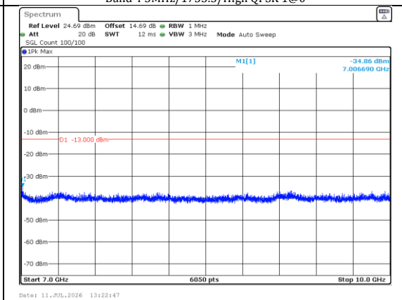
7000.0MHz-10000.0MHz Band 4 3MHz/1753.5/High QPSK 1@0
