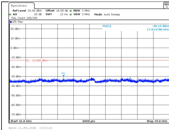
16000.0MHz-19000.0MHz Band 4 10MHz/1750.0/High 16QAM 1@0
