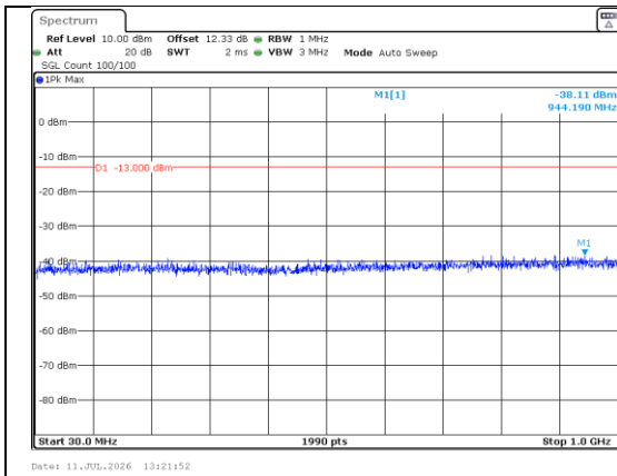
30.0MHz-1000.0MHz Band 4 3MHz/1753.5/High QPSK 1@0
