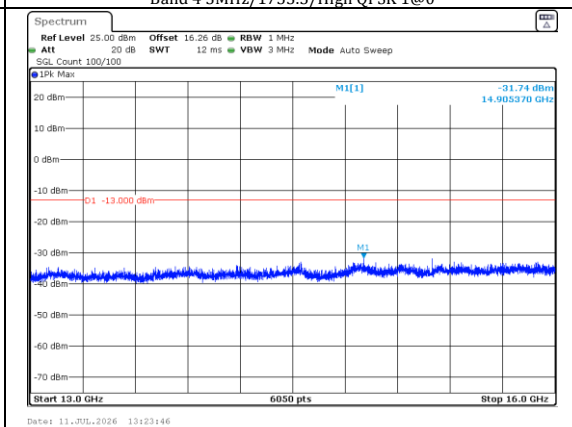
13000.0MHz-16000.0MHz Band 4 3MHz/1753.5/High QPSK 1@0
