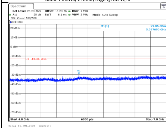
4000.0MHz-7000.0MHz Band 4 3MHz/1753.5/High QPSK 1@0
