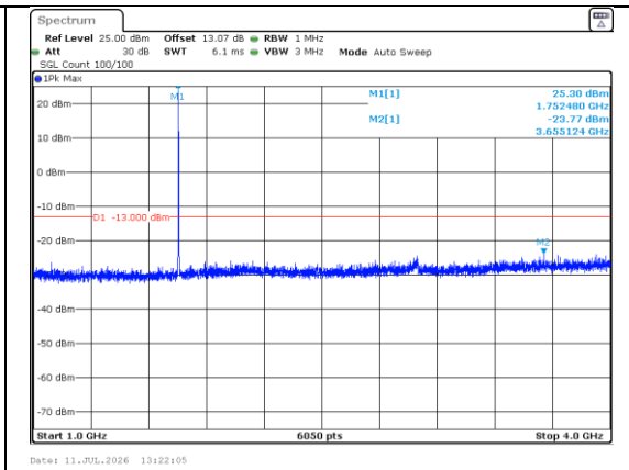
1000.0MHz-4000.0MHz Band 4 3MHz/1753.5/High QPSK 1@0
