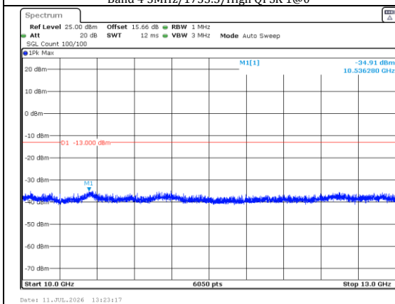
10000.0MHz-13000.0MHz Band 4 3MHz/1753.5/High QPSK 1@0
