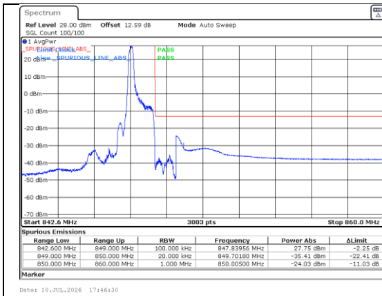
Band 5 1.4MHz/848.3/High QPSK 1@0
