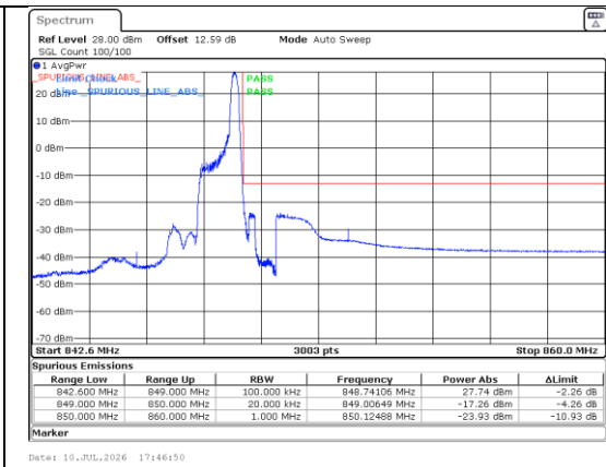
Band 5 1.4MHz/848.3/High QPSK 1@5
