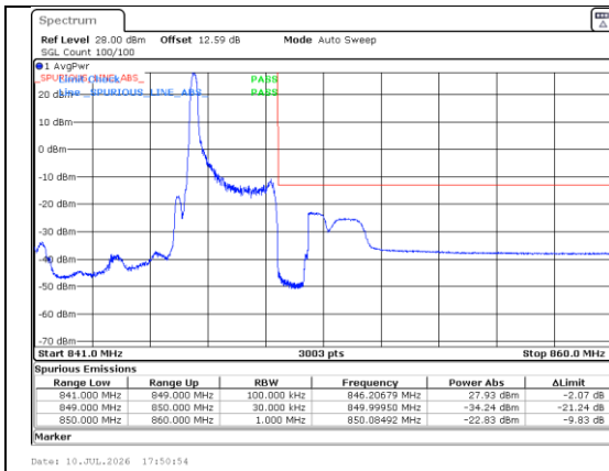
Band 5 3MHz/847.5/High QPSK 1@0
