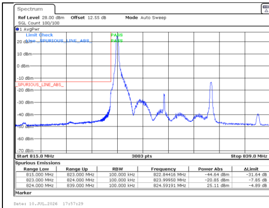
Band 5 10MHz/829.0/Low QPSK 1@0
