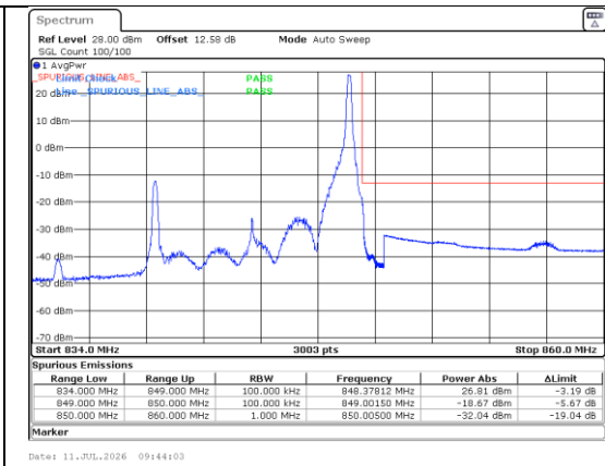
Band 5 10MHz/844.0/High QPSK 1@49
