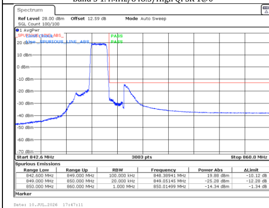
Band 5 1.4MHz/848.3/High QPSK 6@0
