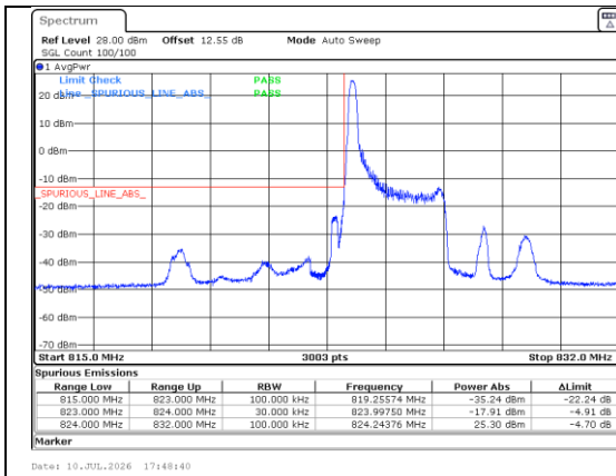
Band 5 3MHz/825.5/Low QPSK 1@0
