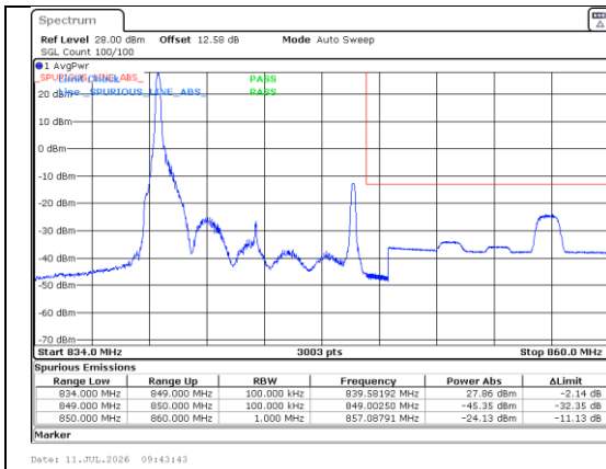
Band 5 10MHz/844.0/High QPSK 1@0
