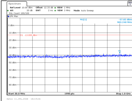
30.0MHz-1000.0MHz Band 66 10MHz/1775.0/High 16QAM 1@0
