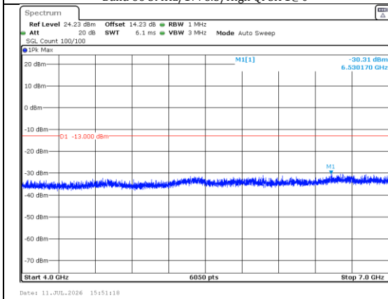
4000.0MHz-7000.0MHz Band 66 3MHz/1778.5/High QPSK 1@0
