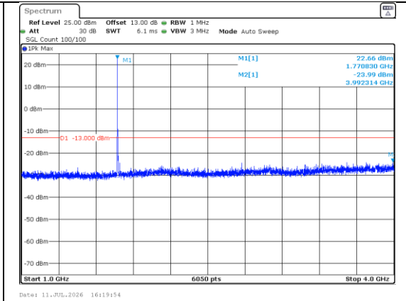
1000.0MHz-4000.0MHz Band 66 10MHz/1775.0/High 16QAM 1@0
