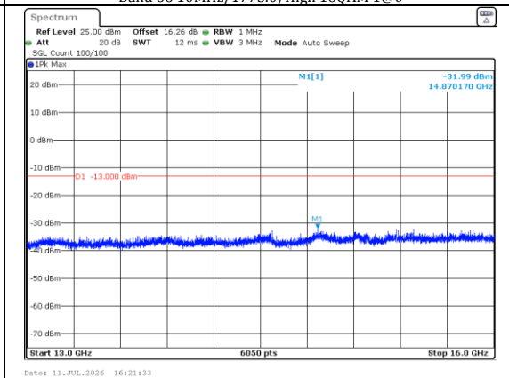
13000.0MHz-16000.0MHz Band 66 10MHz/1775.0/High 16QAM 1@0
