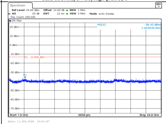
7000.0MHz-10000.0MHz Band 66 3MHz/1778.5/High QPSK 1@0
