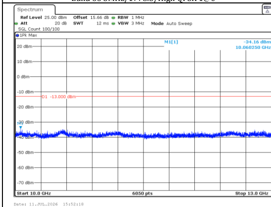
10000.0MHz-13000.0MHz Band 66 3MHz/1778.5/High QPSK 1@0
