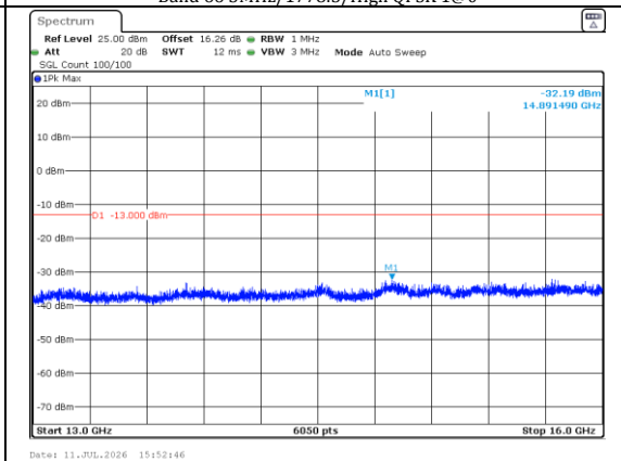
13000.0MHz-16000.0MHz Band 66 3MHz/1778.5/High QPSK 1@0
