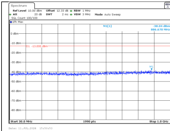
30.0MHz-1000.0MHz Band 66 3MHz/1778.5/High QPSK 1@0
