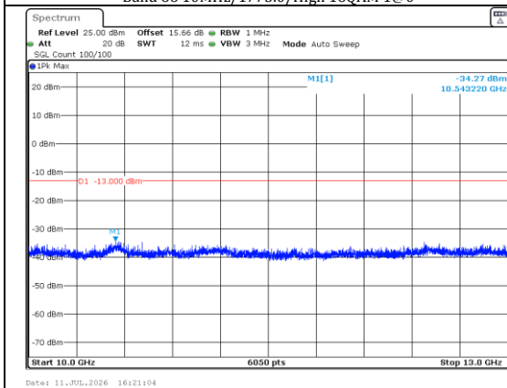
10000.0MHz-13000.0MHz Band 66 10MHz/1775.0/High 16QAM 1@0
