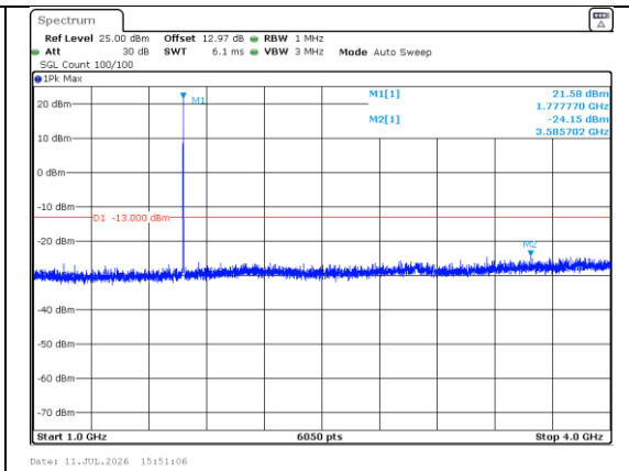
1000.0MHz-4000.0MHz Band 66 3MHz/1778.5/High QPSK 1@0
