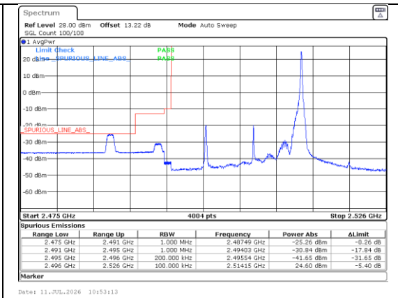
Band 7 15MHz/2507.5/Low QPSK 1@74
