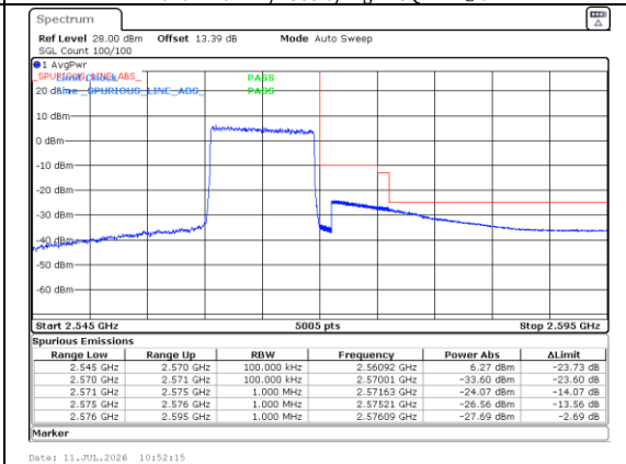
Band 7 10MHz/2565.0/High 16QAM 50@0
