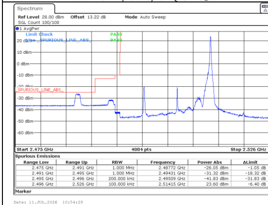
Band 7 15MHz/2507.5/Low 16QAM 1@74
