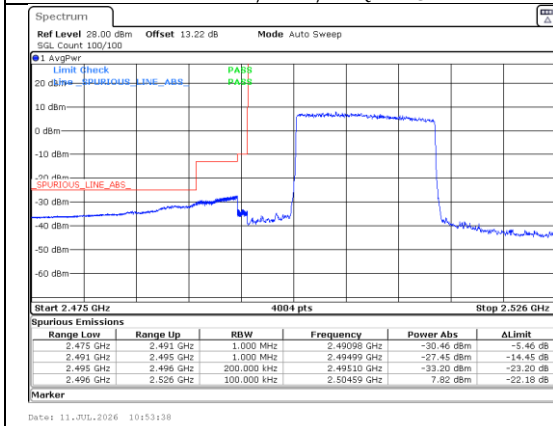
Band 7 15MHz/2507.5/Low QPSK 75@0
