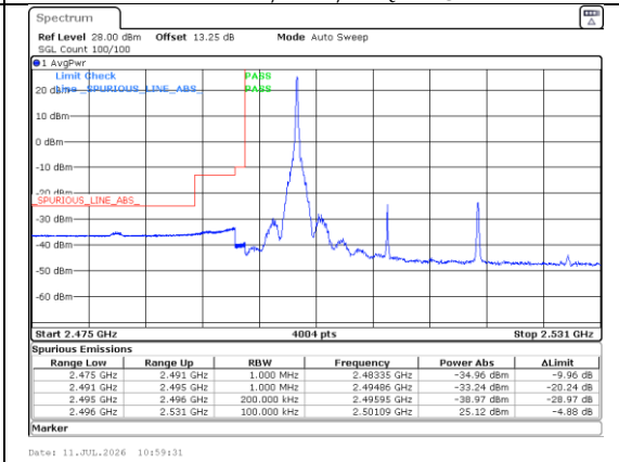
Band 7 20MHz/2510.0/Low 16QAM 1@0
