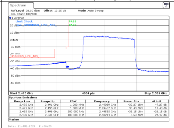
Band 7 20MHz/2510.0/Low 16QAM 1@0
