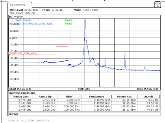
Band 7 15MHz/2507.5/Low 16QAM 1@0
