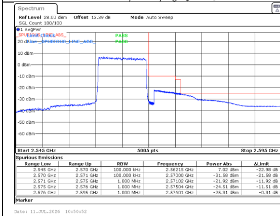
Band 7 10MHz/2565.0/High QPSK 50@0
