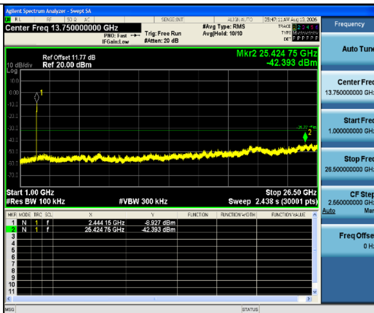
11AX40SISO-Ant1-2452-0~Reference-PASS
