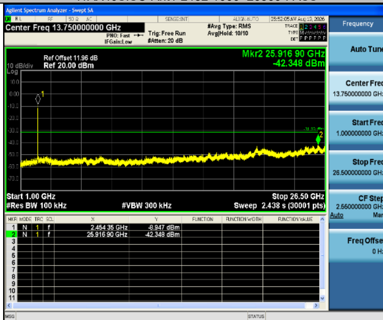
11B-Ant1-2412-0~Reference-PASS
