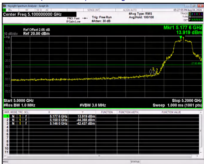
(802.11ac40) Band Edge, Left Side
