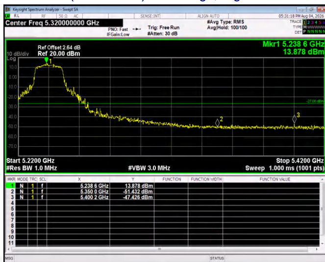
(802.11ac40) Band Edge, Right Side
