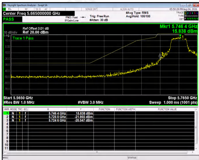
(802.11n20) Band Edge, Left Side
