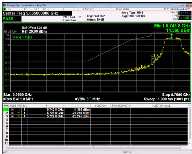
(802.11n40) Band Edge, Left Side
