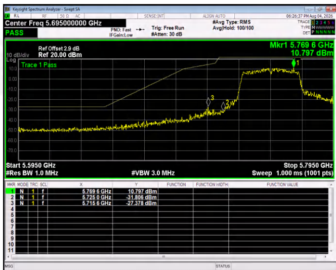
(802.11ac80) Band Edge, Left Side
