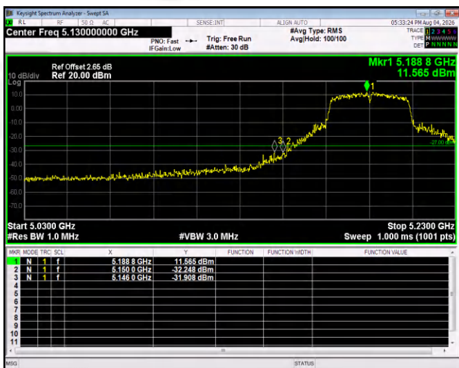
(802.11ac80) Band Edge, Left Side
