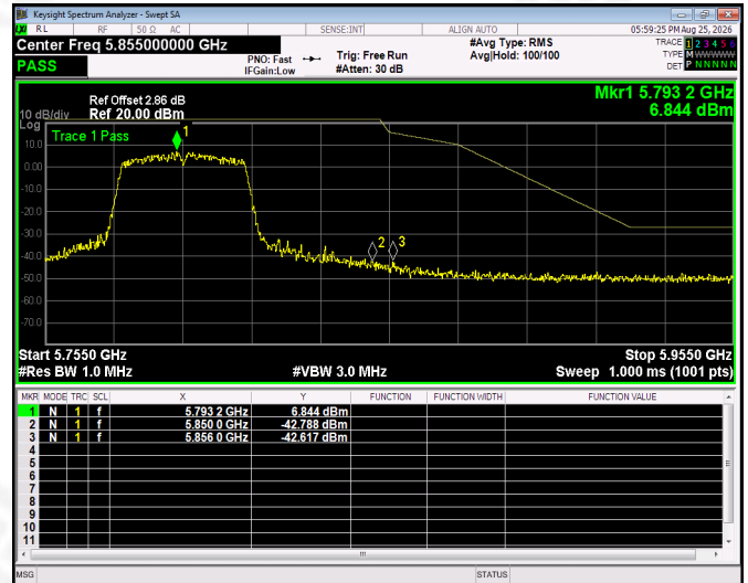
(802.11ac80) Band Edge, Right Side
