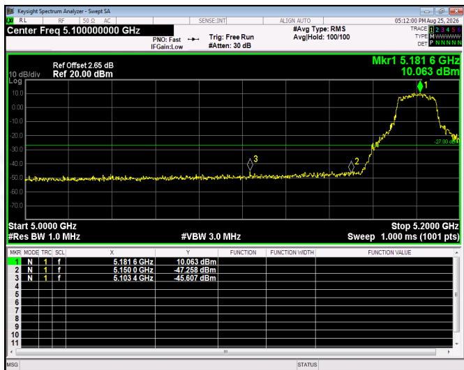
(802.11ac40) Band Edge, Left Side
