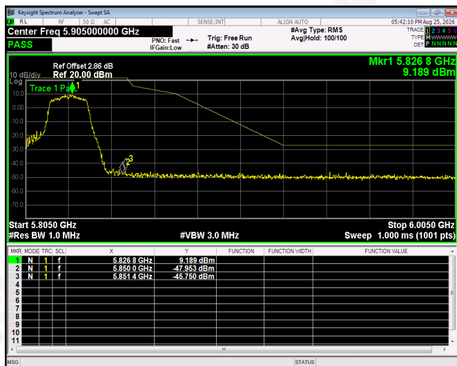
(802.11n40) Band Edge, Right Side
