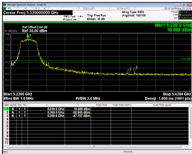
(802.11ac40) Band Edge, Right Side
