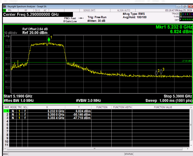
(802.11ac80) Band Edge, Right Side
