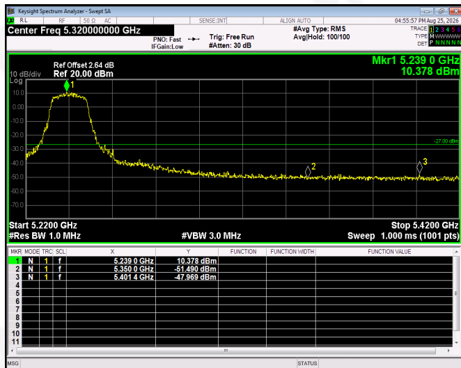
(802.11n20) Band Edge, Right Side
