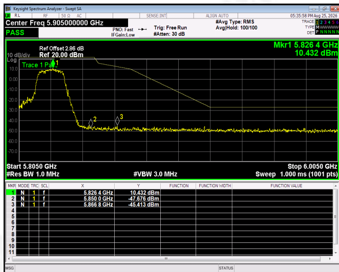
(802.11n20) Band Edge, Right Side
