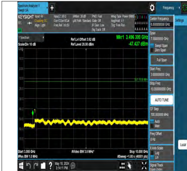
Band12_1.4MHz_QPSK_23017_1RB#0_3000~10000_3000~1000
