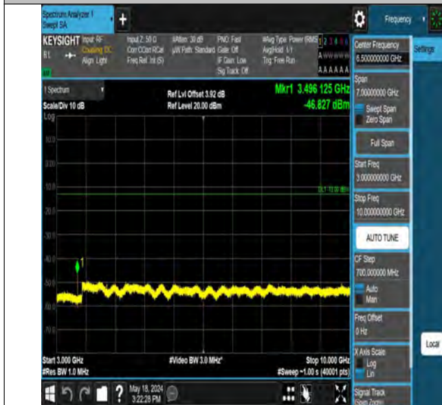
Band12_3MHz_QPSK_23025_1RB#0_3000~10000_3000~10000
