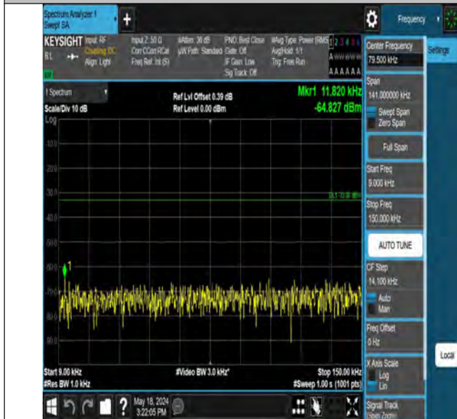
Band12_3MHz_QPSK_23025_1RB#0_0.009~0.15_0.009~0.15
