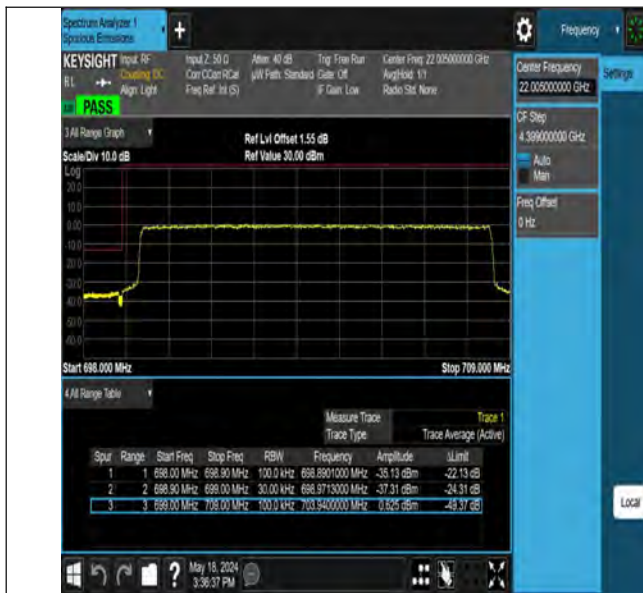
Band12_10MHz_QPSK_23060_50RB#0
