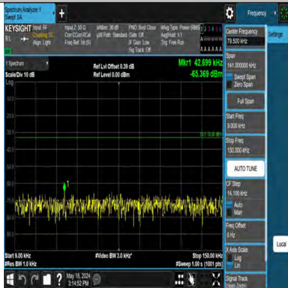
Band12_1.4MHz_QPSK_23095_1RB#0_0.009~0.15_0.009~0.15
