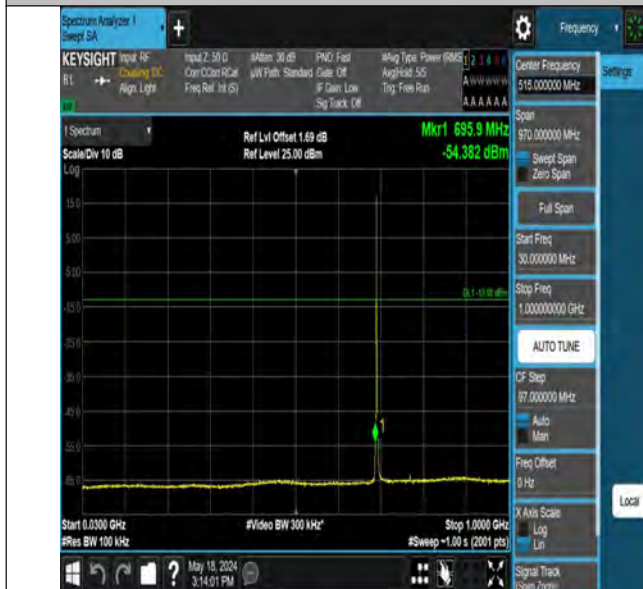
Band12_1.4MHz_QPSK_23017_1RB#0_30~1000_30~1000
