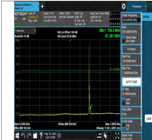
Band12_3MHz_QPSK_23025_1RB#0_30~1000_30~1000
