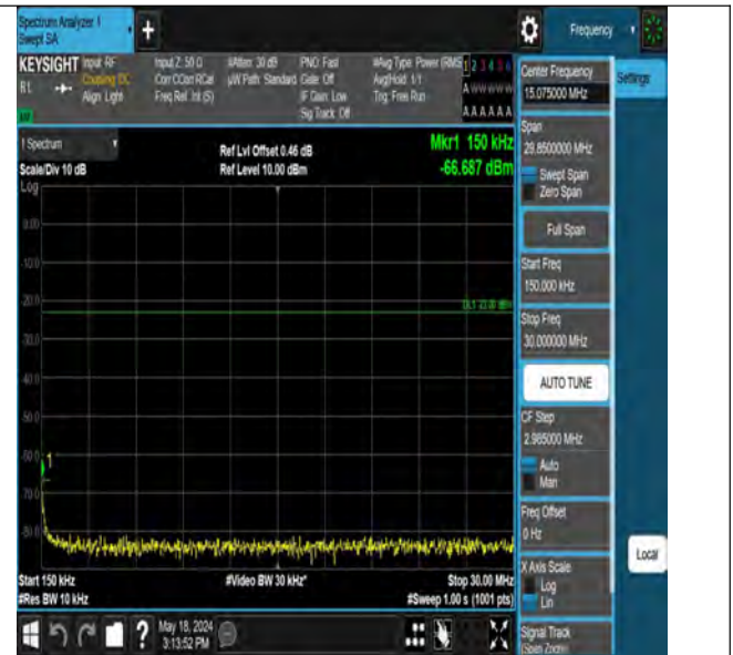
Band12_1.4MHz_QPSK_23017_1RB#0_0.15~30_0.15~30
