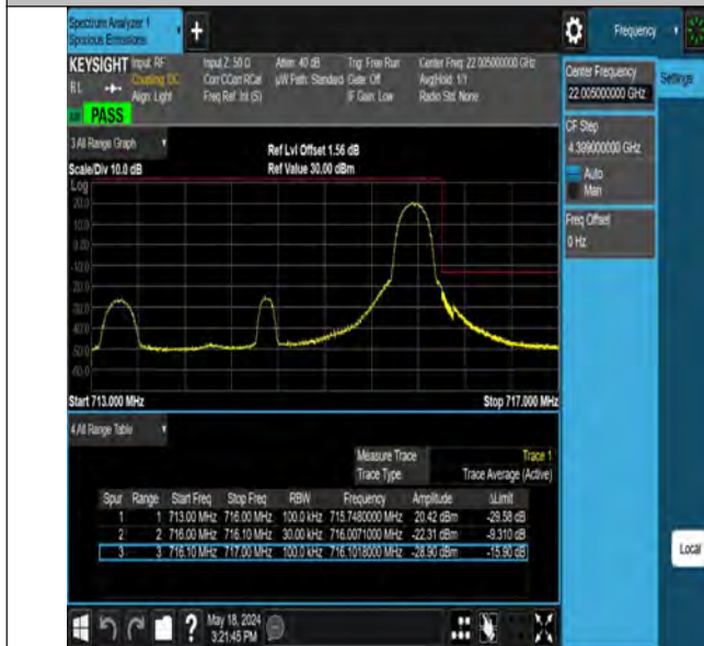
Band12_3MHz_QPSK_23165_1RB#14
