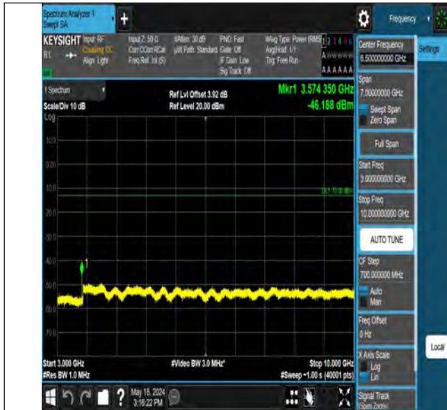
Band12_1.4MHz_QPSK_23173_1RB#0_3000~10000_3000~1000
