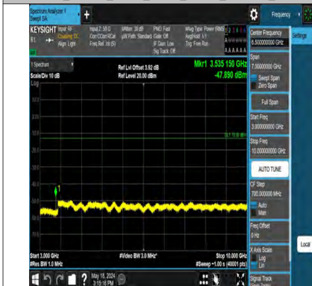
Band12_1.4MHz_QPSK_23095_1RB#0_3000~10000_3000~1000
