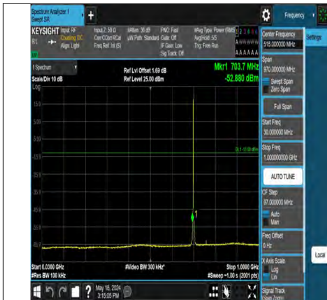
Band12_1.4MHz_QPSK_23095_1RB#0_30~1000_30~1000
