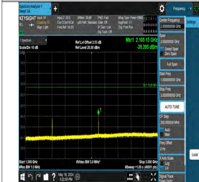
Band12_3MHz_QPSK_23025_1RB#14_1000~3000_1000~3000
