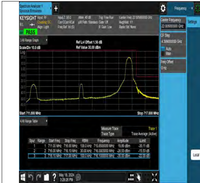
Band12_5MHz_QPSK_23155_1RB#24
