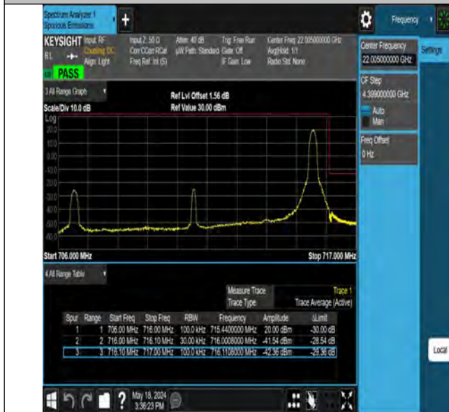
Band12_10MHz_QPSK_23130_1RB#49
