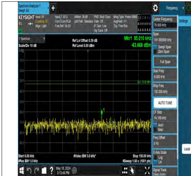
Band12_1.4MHz_QPSK_23017_1RB#0_0.009~0.15_0.009~0.15
