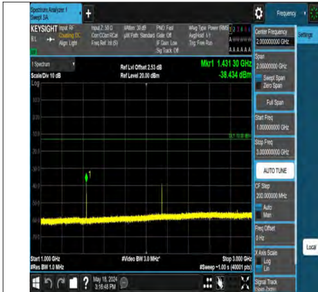
Band12_1.4MHz_QPSK_23173_1RB#5_1000~3000_1000~3000
