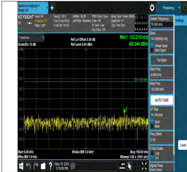
Band12_1.4MHz_QPSK_23173_1RB#0_0.009~0.15_0.009~0.15
