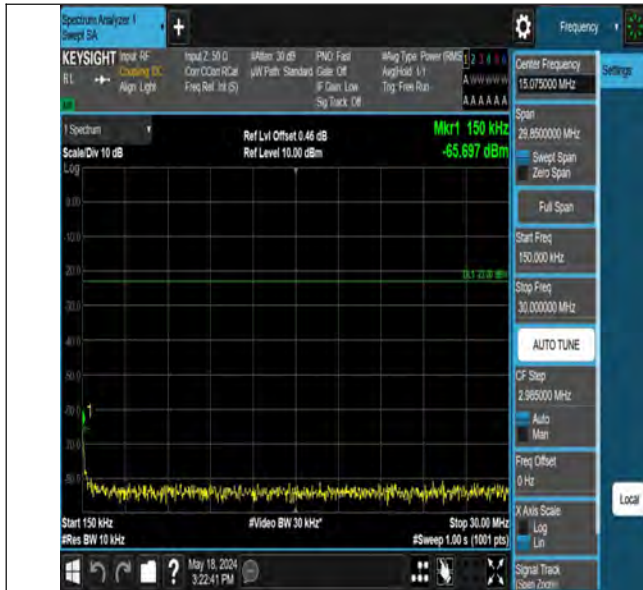
Band12_3MHz_QPSK_23025_1RB#14_0.15~30_0.15~30
