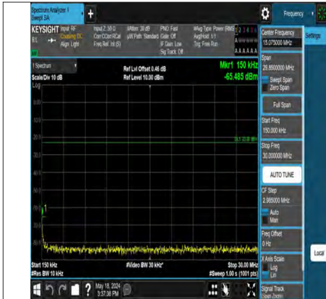
Band12_10MHz_QPSK_23060_1RB#49_0.15~30_0.15~30
