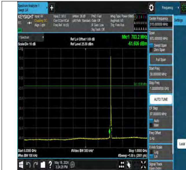
Band12_3MHz_QPSK_23165_1RB#0_30~1000_30~1000
