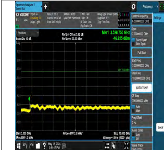
Band12_5MHz_QPSK_23095_1RB#0_3000~10000_3000~10000
