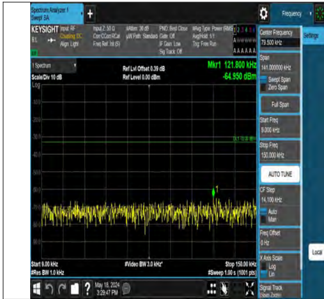
Band12_5MHz_QPSK_23035_1RB#0_0.009~0.15_0.009~0.15
