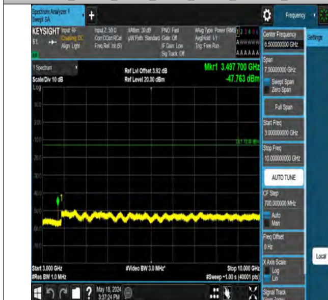
Band12_10MHz_QPSK_23060_1RB#0_3000~10000_3000~1000
