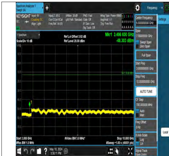
Band12_5MHz_QPSK_23035_1RB#0_3000~10000_3000~10000
