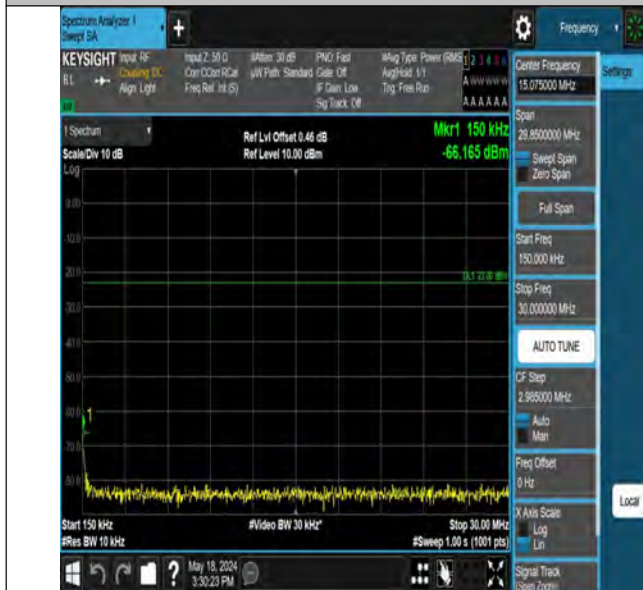
Band12_5MHz_QPSK_23035_1RB#24_0.15~30_0.15~30
