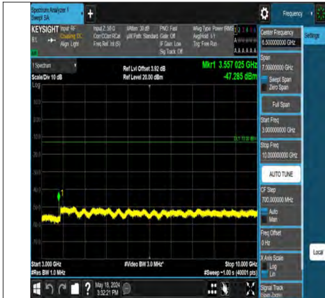
Band12_5MHz_QPSK_23155_1RB#0_3000~10000_3000~10000
