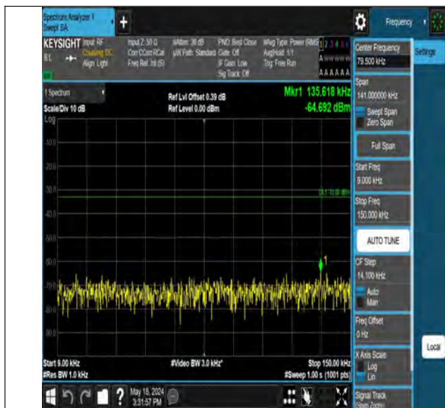
Band12_5MHz_QPSK_23155_1RB#0_0.009~0.15_0.009~0.15
