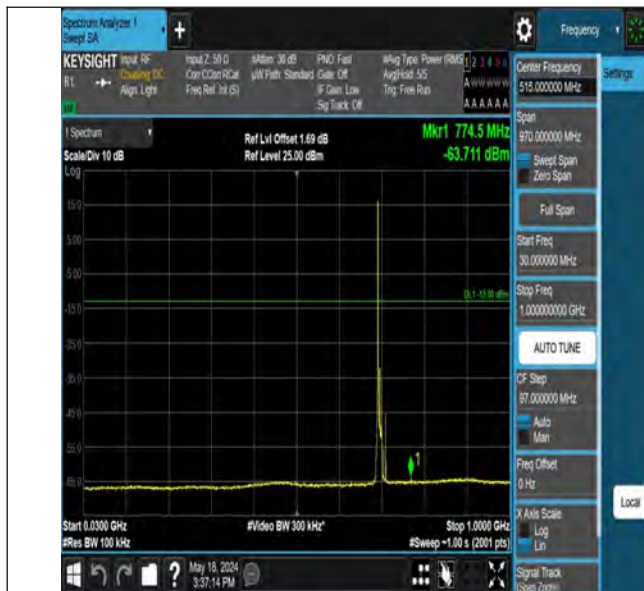
Band12_10MHz_QPSK_23060_1RB#0_30~1000_30~1000
