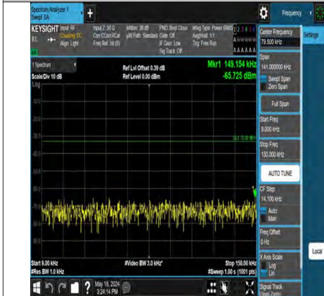
Band12_3MHz_QPSK_23165_1RB#0_0.009~0.15_0.009~0.15
