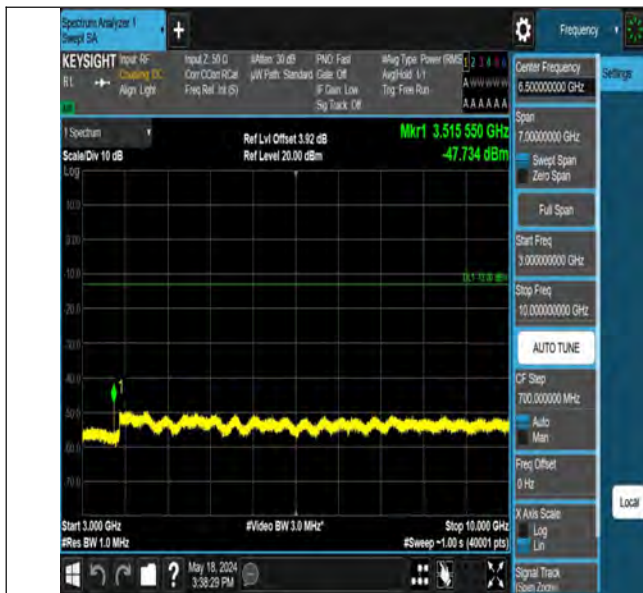
Band12_10MHz_QPSK_23095_1RB#0_3000~10000_3000~1000
