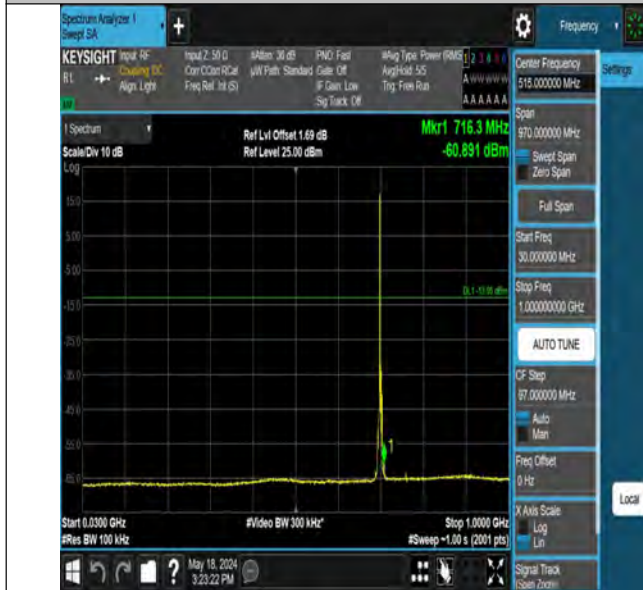
Band12_3MHz_QPSK_23095_1RB#0_30~1000_30~1000
