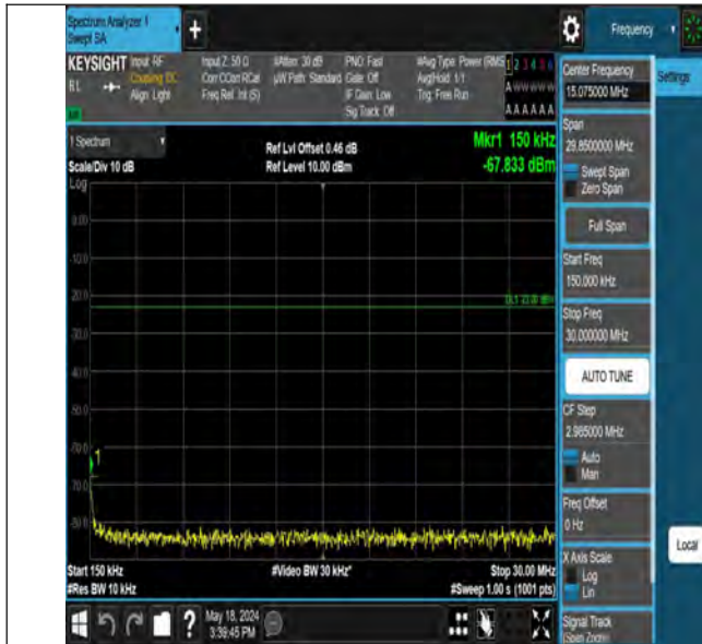
Band12_10MHz_QPSK_23130_1RB#49_0.15~30_0.15~30
