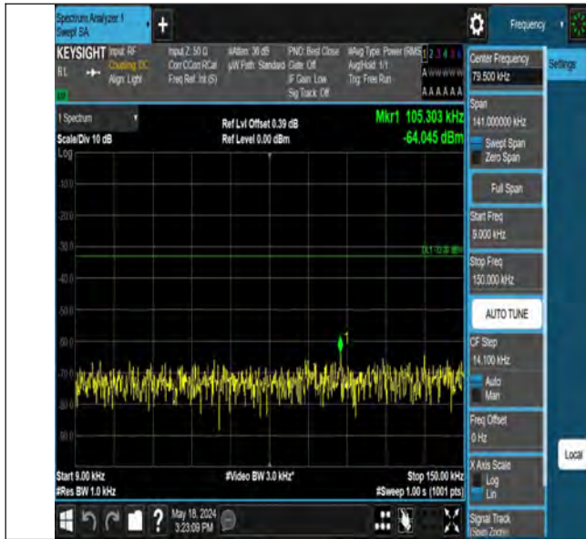
Band12_3MHz_QPSK_23095_1RB#0_0.009~0.15_0.009~0.15
