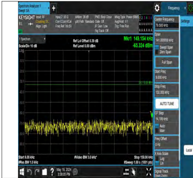
Band12_10MHz_QPSK_23095_1RB#0_0.009~0.15_0.009~0.15
