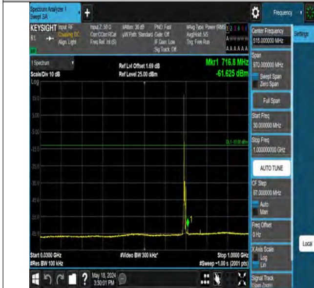
Band12_5MHz_QPSK_23035_1RB#0_30~1000_30~1000
