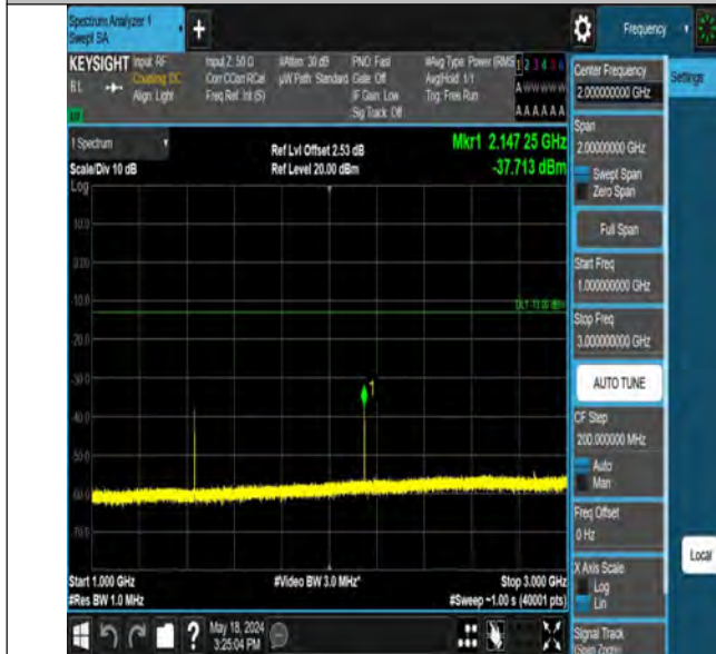
Band12_3MHz_QPSK_23165_1RB#14_1000~3000_1000~3000
