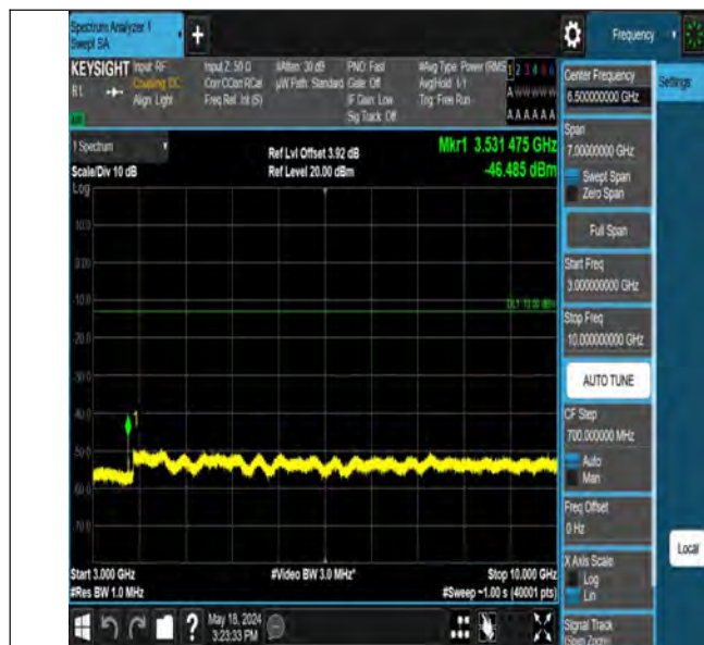
Band12_3MHz_QPSK_23095_1RB#0_3000~10000_3000~10000
