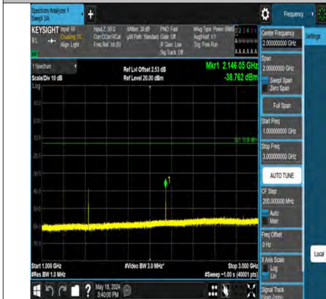
Band12_10MHz_QPSK_23130_1RB#49_1000~3000_1000~3000
