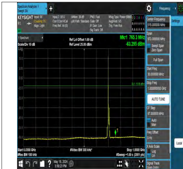
Band12_10MHz_QPSK_23130_1RB#0_30~1000_30~1000
