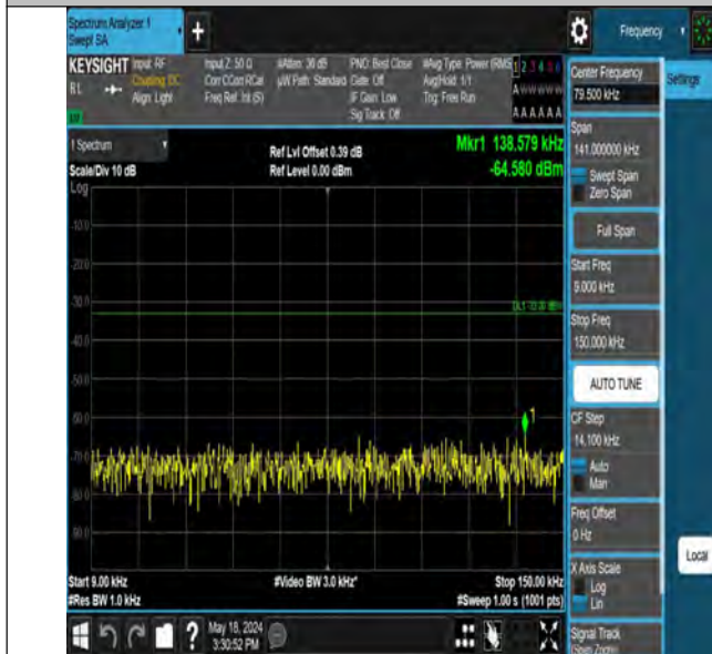
Band12_5MHz_QPSK_23095_1RB#0_0.009~0.15_0.009~0.15
