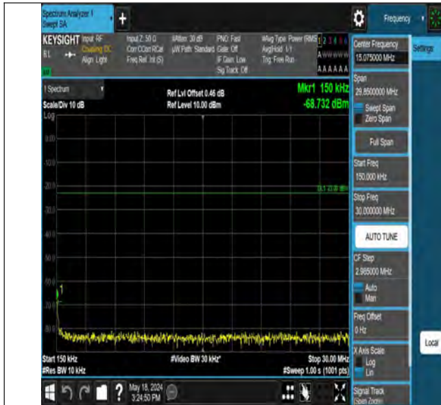
Band12_3MHz_QPSK_23165_1RB#14_0.15~30_0.15~30
