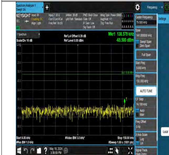
Band12_10MHz_QPSK_23060_1RB#0_0.009~0.15_0.009~0.15
