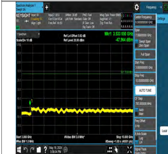
Band12_10MHz_QPSK_23130_1RB#0_3000~10000_3000~1000
