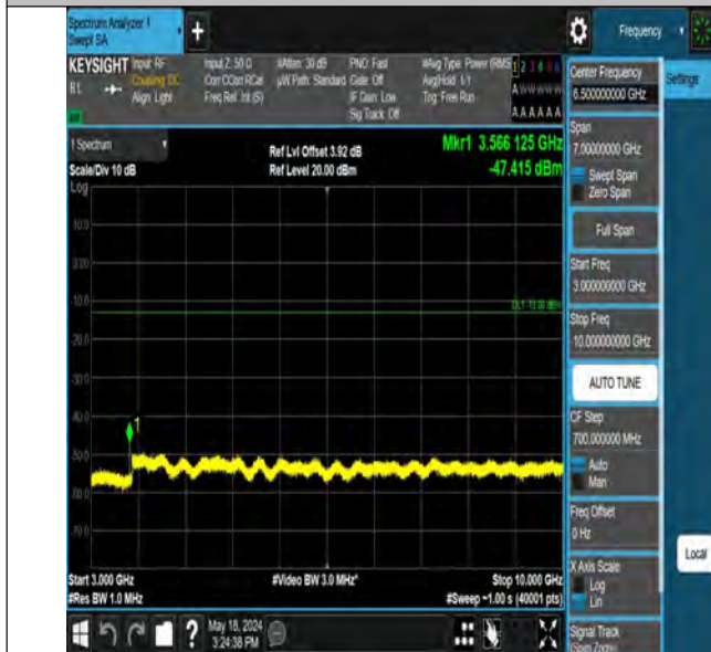
Band12_3MHz_QPSK_23165_1RB#0_3000~10000_3000~10000
