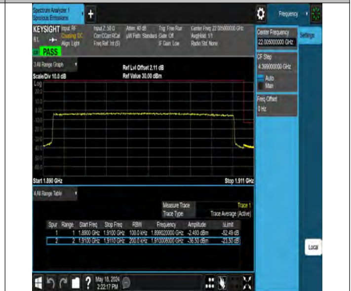
Band2_20MHz_QPSK_19100_100RB#0
