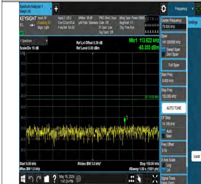
Band2_1.4MHz_QPSK_18900_1RB#0_0.009~0.15_0.009~0.15
