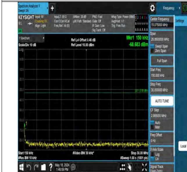
Band2_1.4MHz_QPSK_18607_1RB#5_0.15~30_0.15~30
