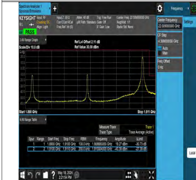
Band2_20MHz_QPSK_19100_1RB#99
