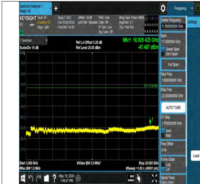
Band2_1.4MHz_QPSK_18607_1RB#0_3000~20000_3000~20000
