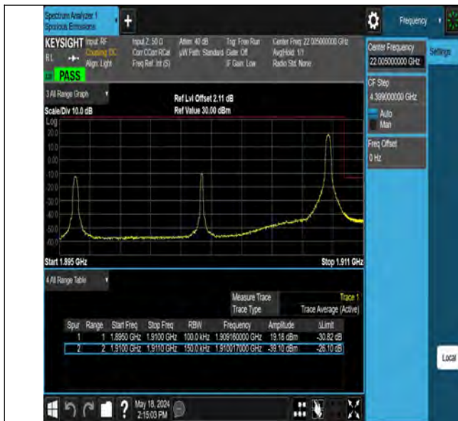
Band2_15MHz_QPSK_19125_1RB#74
