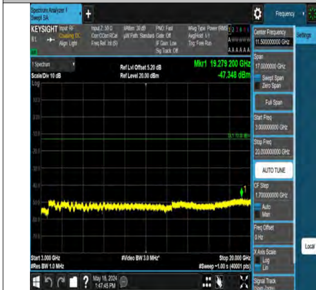
Band2_1.4MHz_QPSK_18900_1RB#0_3000~20000_3000~20000
