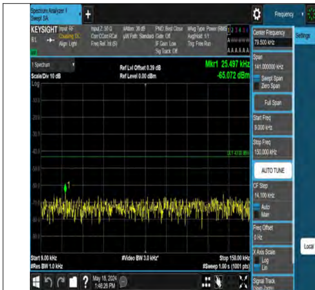
Band2_1.4MHz_QPSK_18607_1RB#0_0.009~0.15_0.009~0.15
