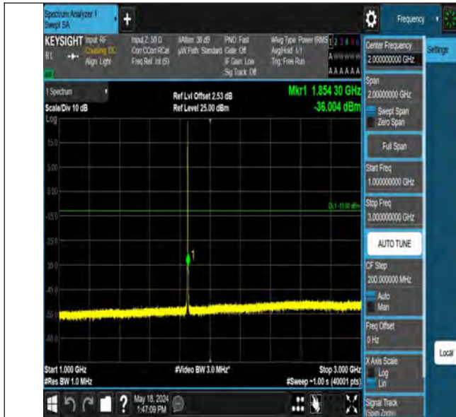
Band2_1.4MHz_QPSK_18607_1RB#5_1000~3000_1000~3000
