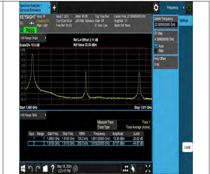
Band2_20MHz_QPSK_19100_1RB#0
