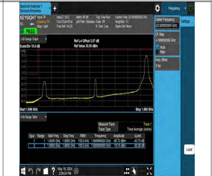
Band2_10MHz_QPSK_18650_1RB#49
