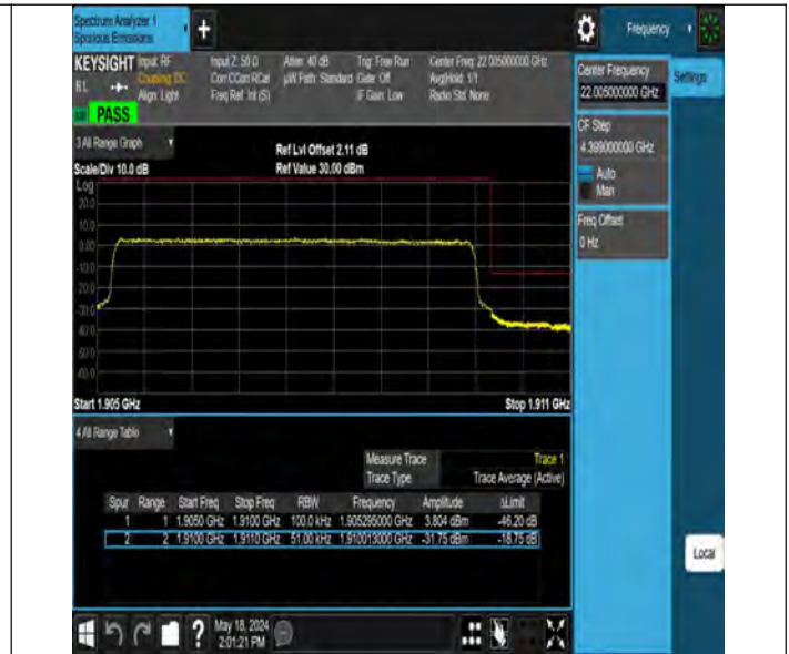
Band2_5MHz_QPSK_19175_25RB#0
