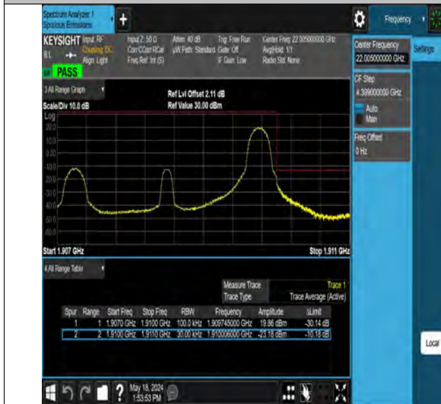
Band2_3MHz_QPSK_19185_1RB#14
