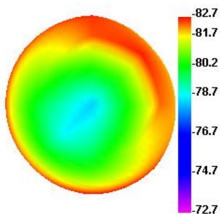
Bluetooth 78 TIS
