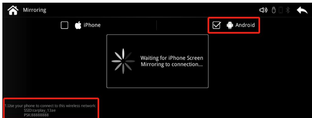
Figure 10: mirroring interface
