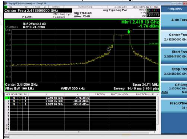
Conducted Spurious Reference,11g,Lowest
