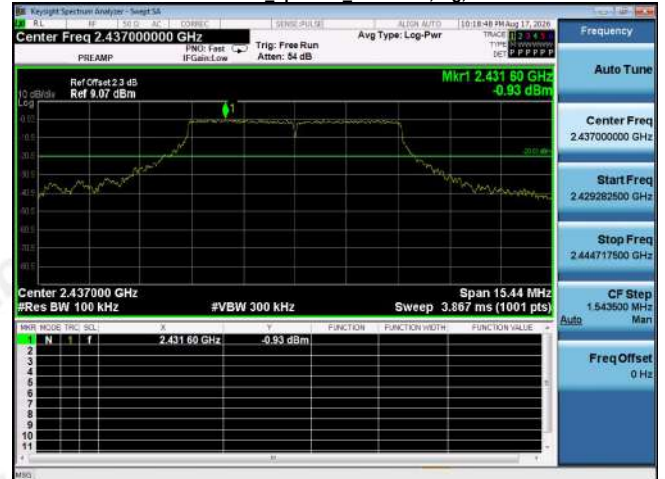
Conducted Spurious Reference,11g,Middle
