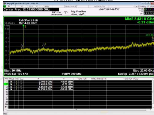
Conducted Spurious,11g,Middle
