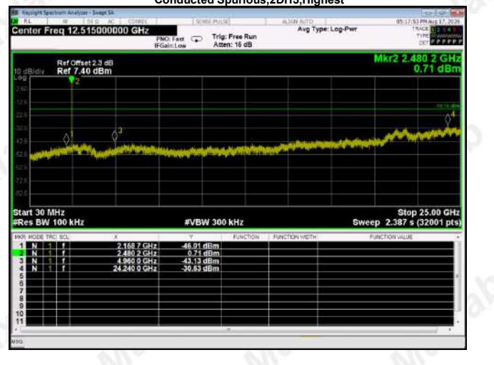
Conducted Spurious,2DH5,Highest
