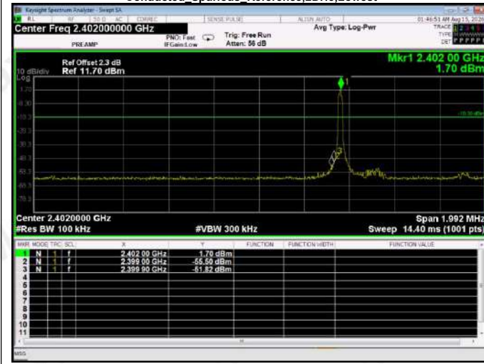
Conducted Spurious Reference,2DH5,Lowest
