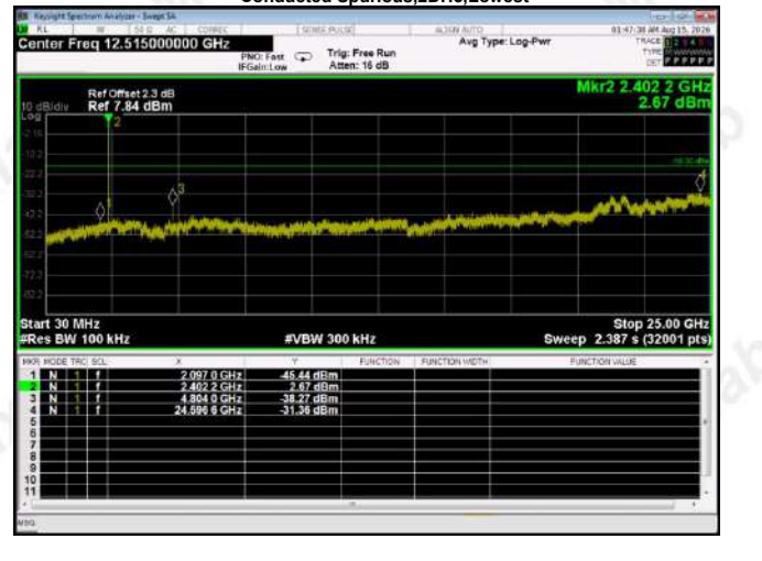
Conducted Spurious,2DH5,Lowest
