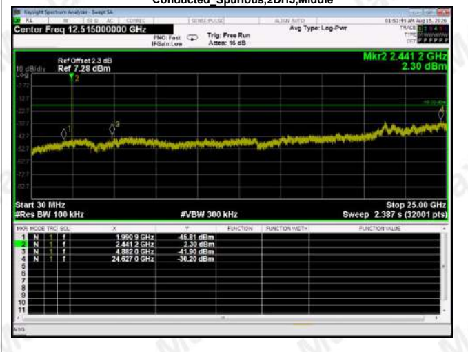
Conducted Spurious,2DH5,Middle
