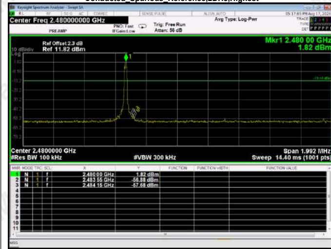
Conducted Spurious Reference,2DH5,Highest
