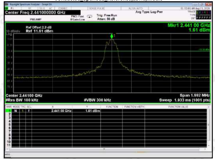
Conducted Spurious Reference,2DH5,Middle
