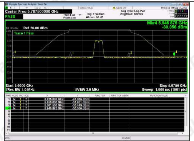
Out Of Band Emission IEEE 802.11a_Channel 157_20MHz
