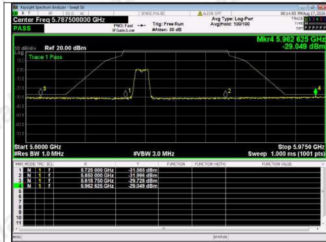
Out Of Band Emission IEEE 802.11a_Channel 149_20MHz
