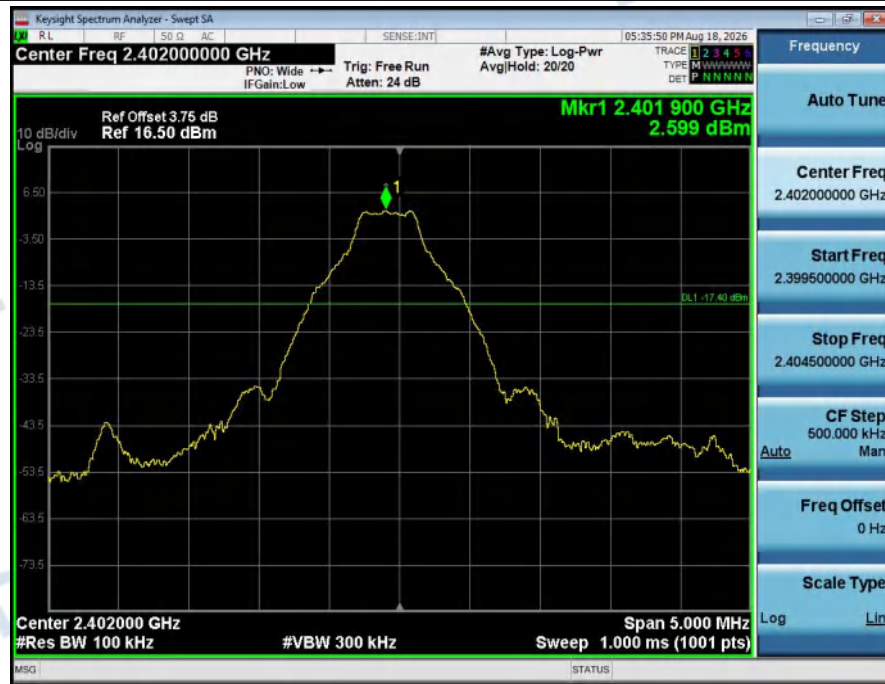
1_Reference_Level_NVNT_ANT1_1-DH5_2402_00
