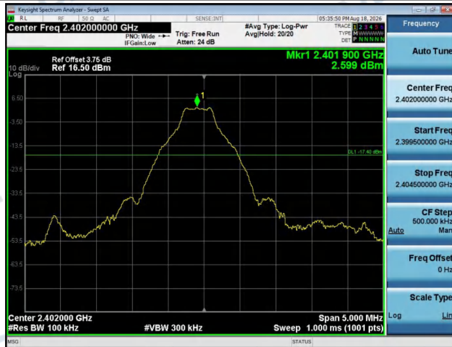
1_Reference_Level_NVNT_ANT1_1-DH5_2402_00
