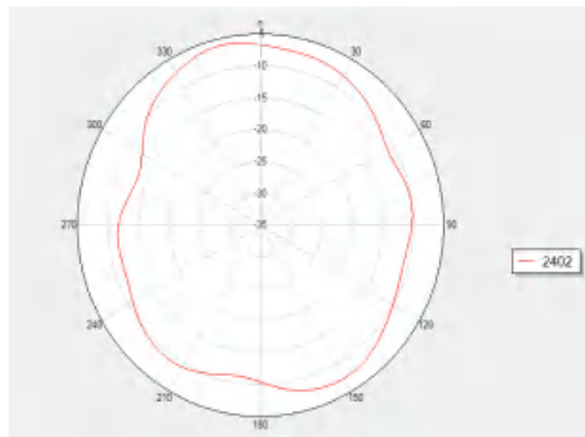
2402MHz XYplane
