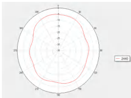
2440MHz XYplane
