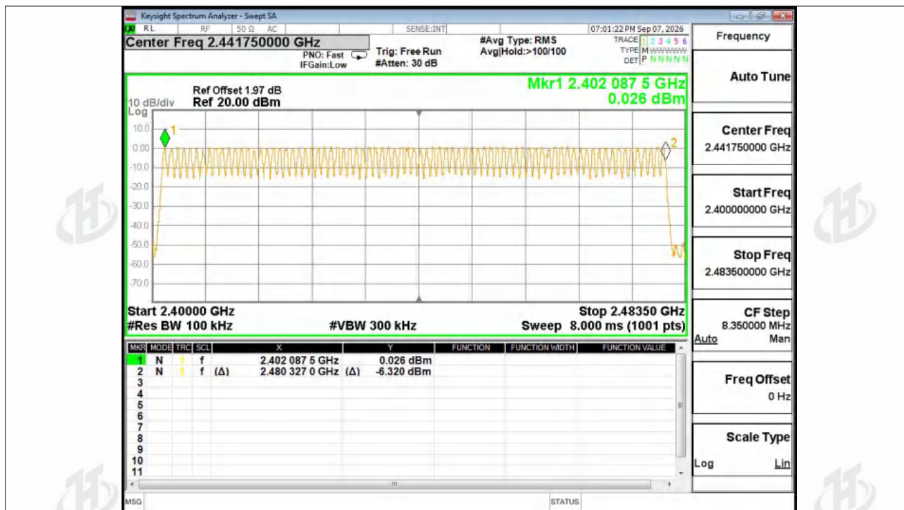
Hopping No. NVNT 1-DH5 2441MHz Ant1
