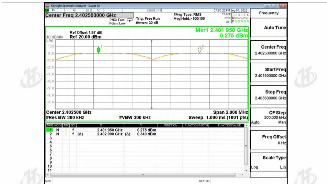
CFS NVNT 1-DH5 2402MHz Ant1
