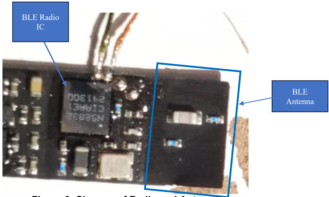
Figure 8. Closeup of Radio and Antenna
