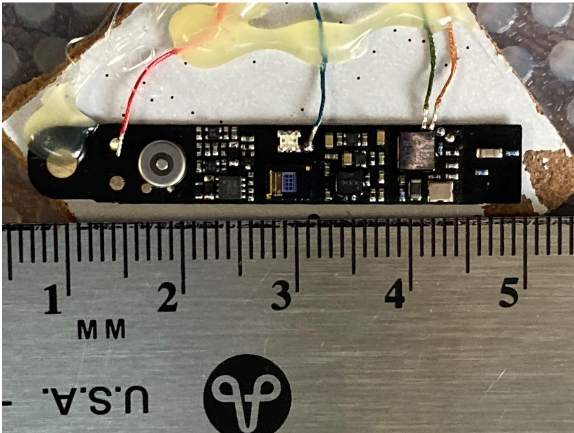
Figure 7. EUT, PCB Front
