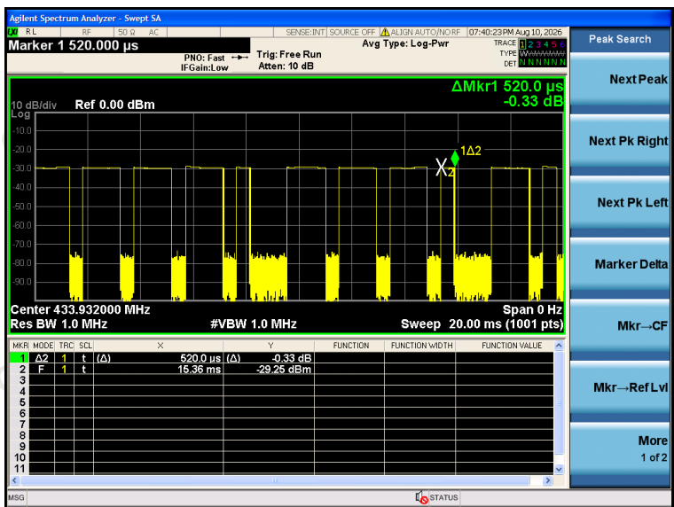
(Time per burst: 0.520 ms*3pcs)
