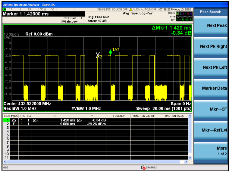
(Time per burst: 1.420ms*22pcs)
