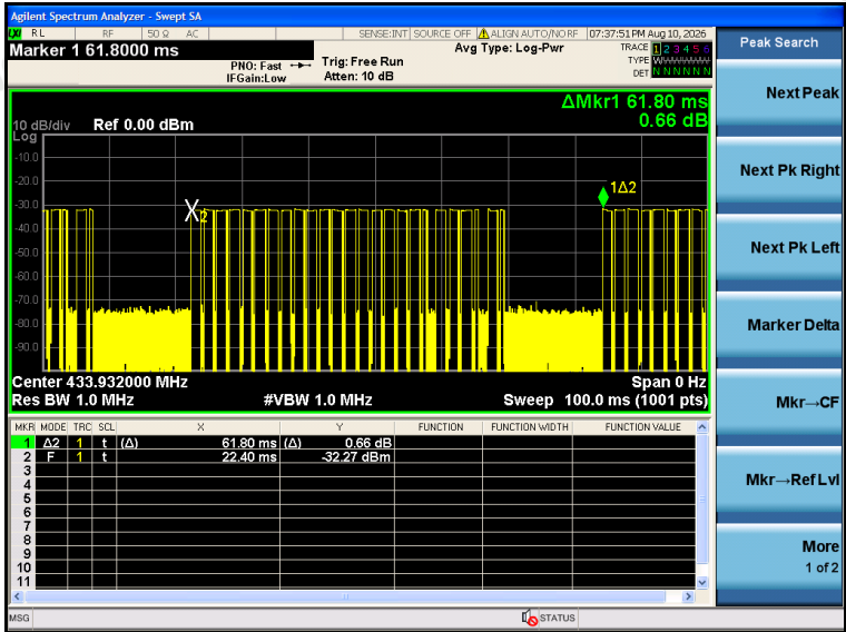
(Transmit cycle 61.8ms)
