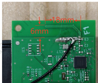
Antenna Dimensions
