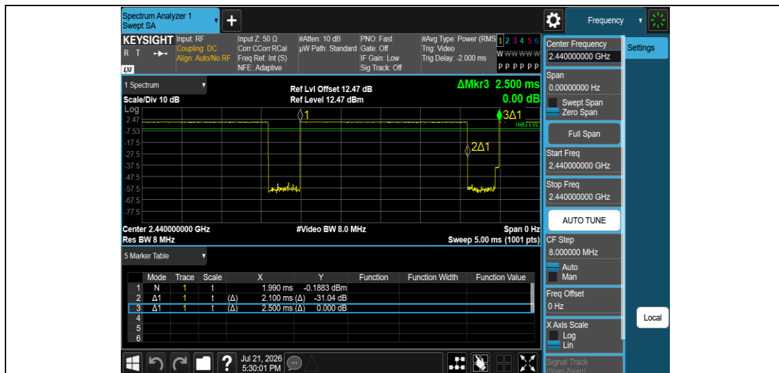
NTNV-BLE_1M-Ant1-2440
