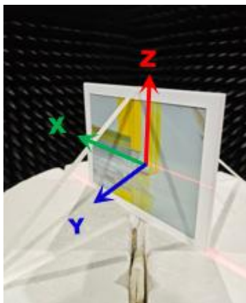
Figure 2: Model F243090-001 Measurement Axes
