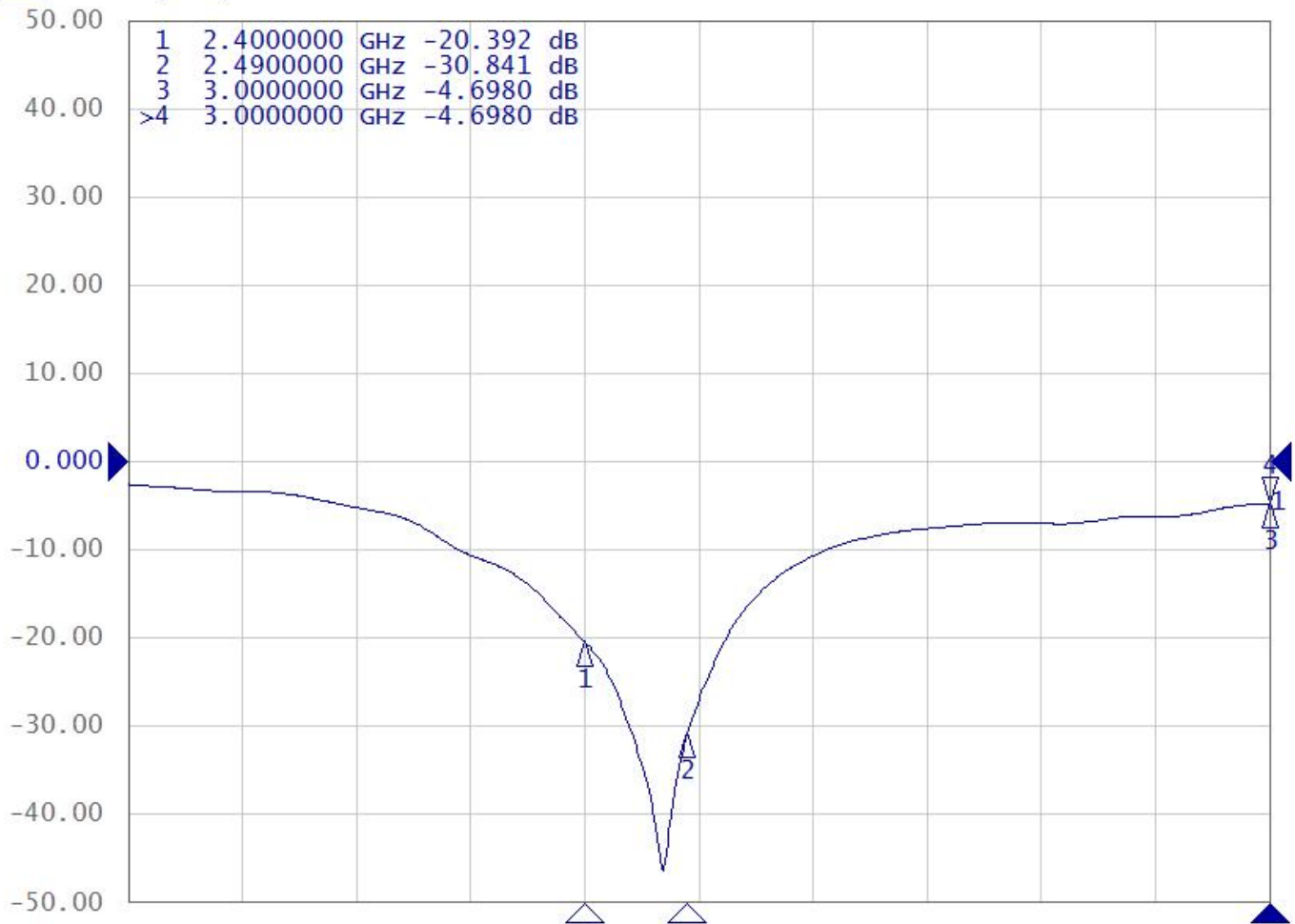
Figure 1: Model F243090-001 Return Loss
