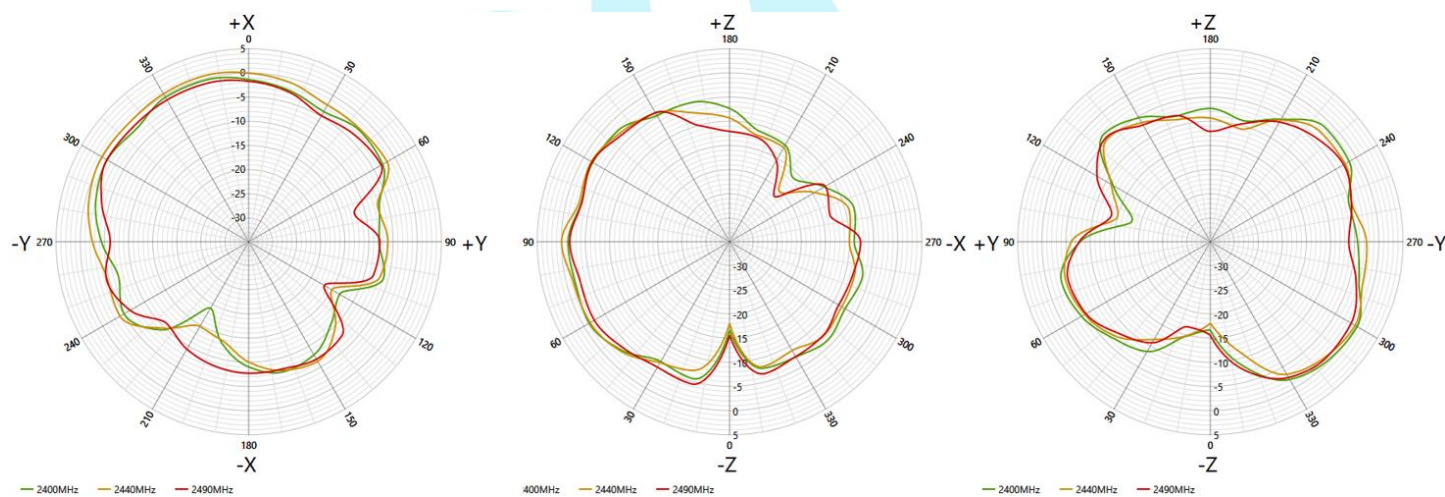
Figure 3: Model F243090-001 Radiation Patterns
