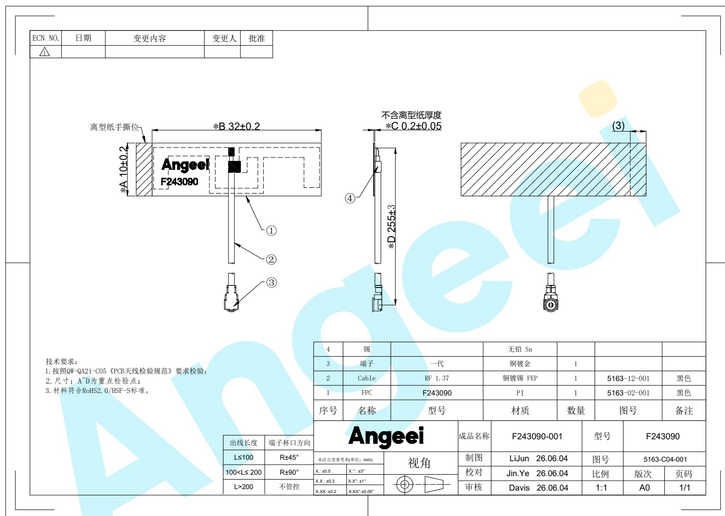
Figure 4: Model F243090-001 Dimensions
