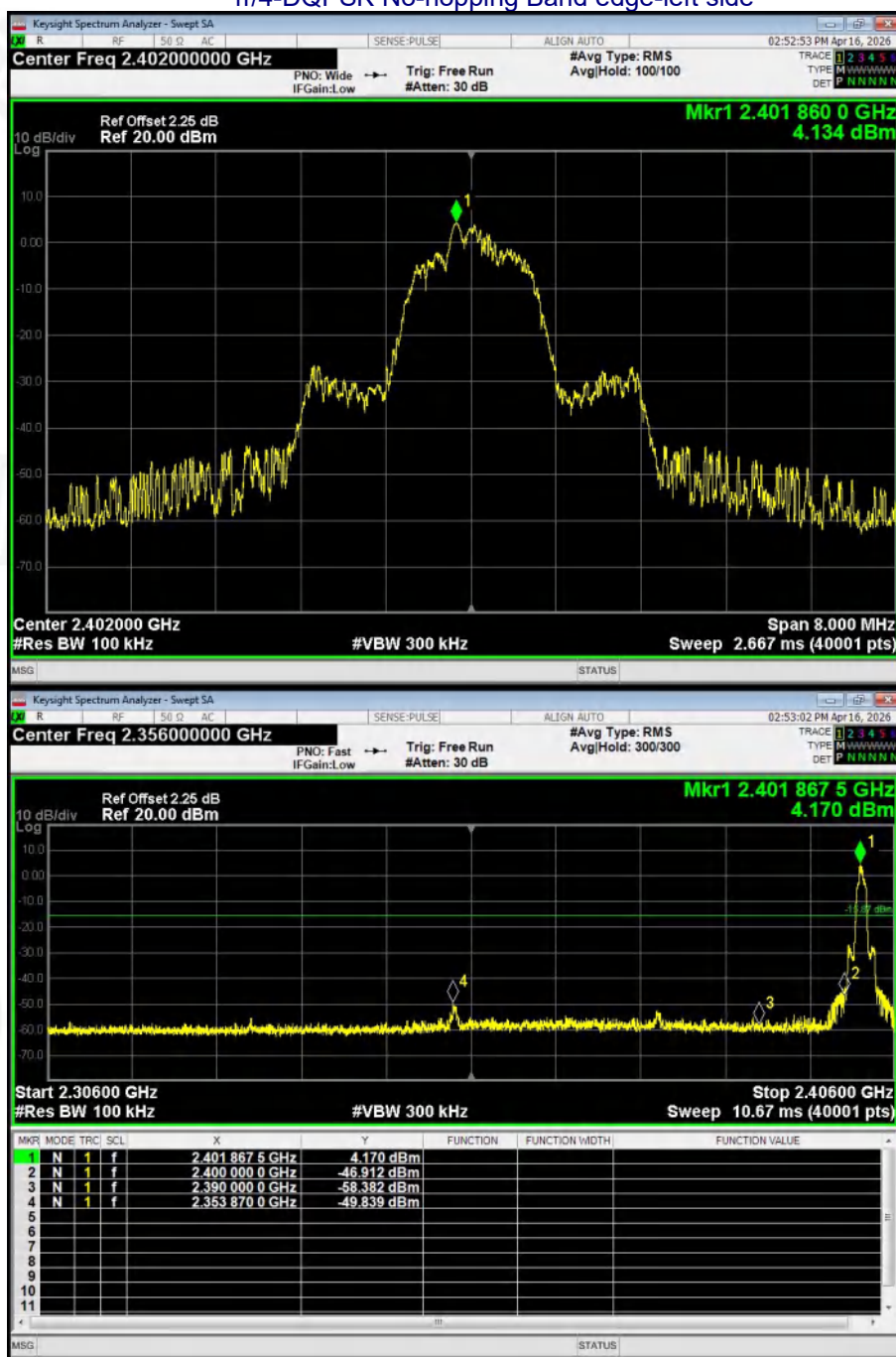
\pi/4 -DQPSK No-hopping Band edge-left side
