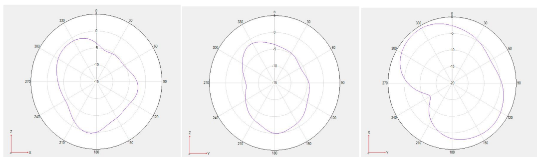
2440MHz (Phi0/Phi90/Theta90)
