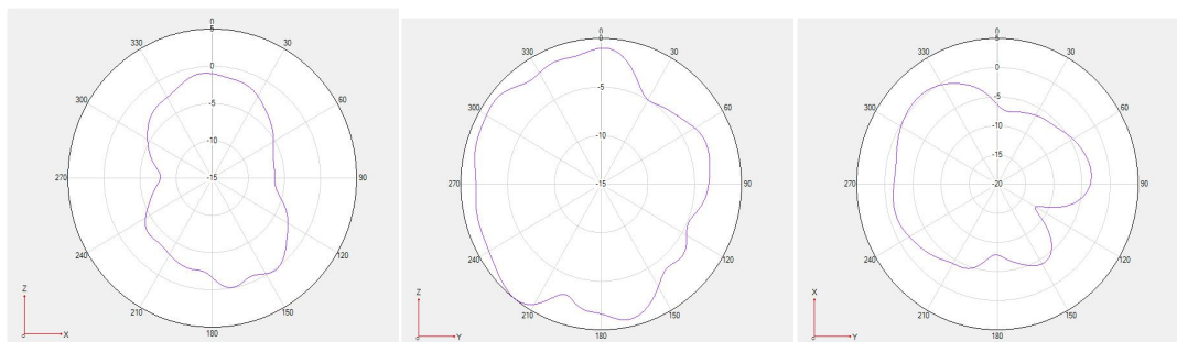
5850MHz (Phi0/Phi90/Theta90)
