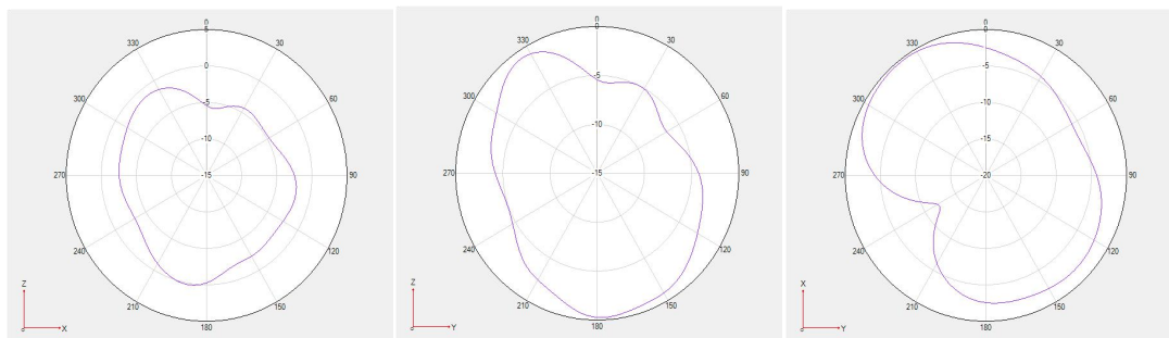
2480MHz (Phi0/Phi90/Theta90)
