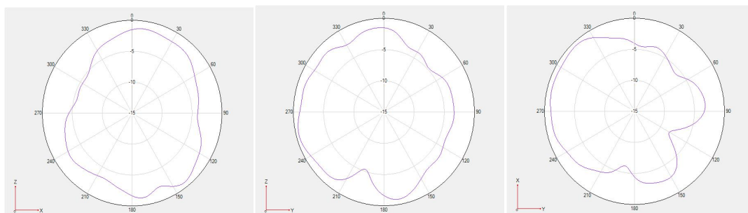
5850MHz (Phi0/Phi90/Theta90)
