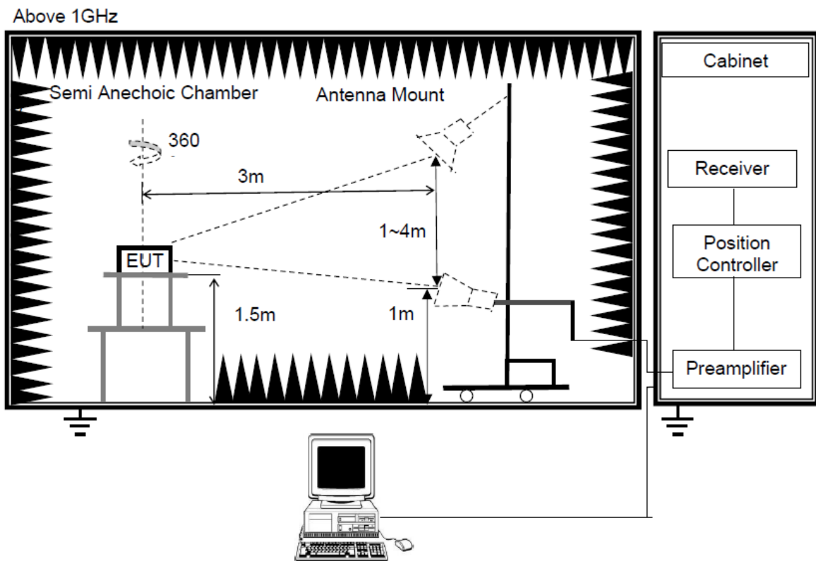
(A) Radiated Emission Test Set-Up, Frequency above 1GHz
