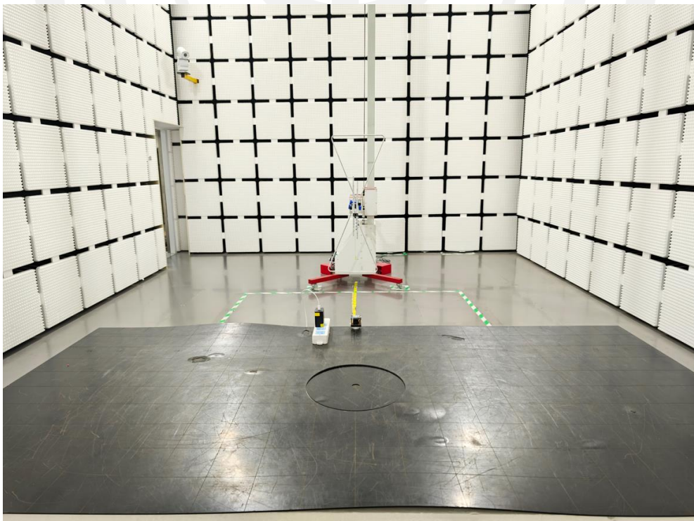
Spurious Radiation Emissions Test (&lt;1G)
