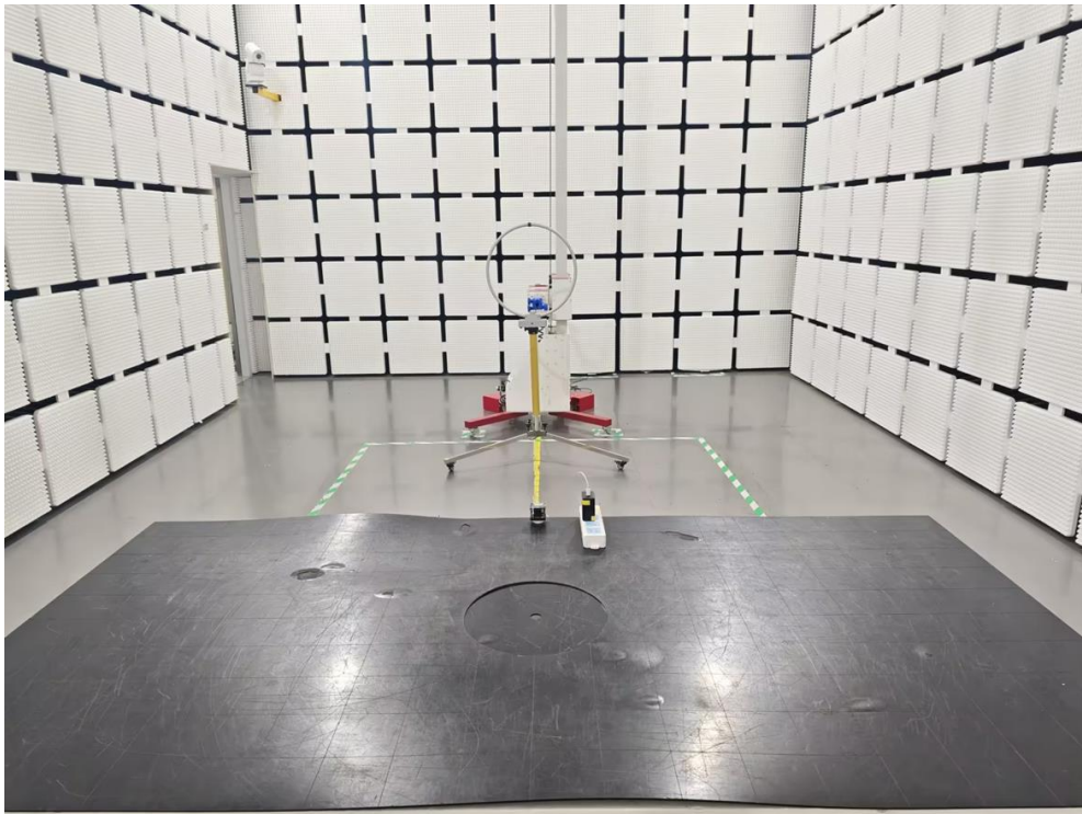
Spurious Radiation Emissions Test (&lt;30M)
