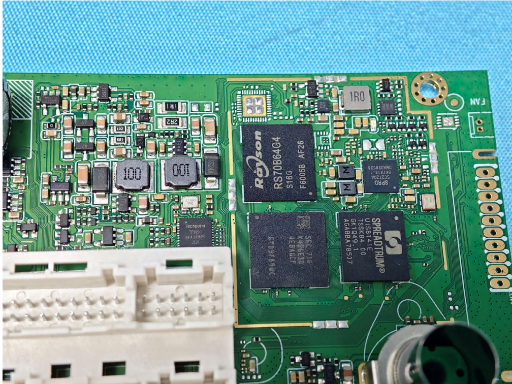
Photo 21 Internal photos of EUT Model: FG-9013 815-A
