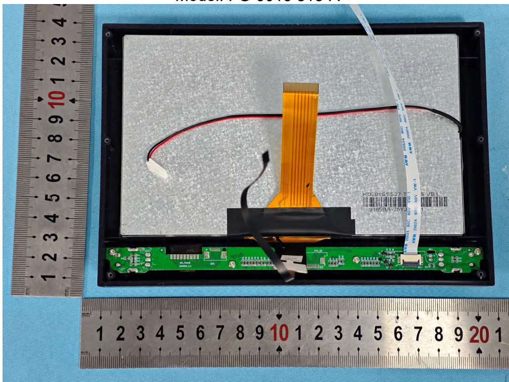
Photo 24 Internal photos of EUT Model: FG-9013 815-A
