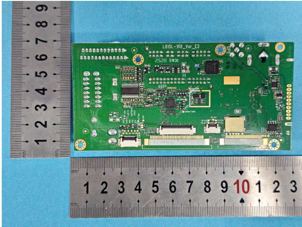
Photo 23 Internal photos of EUT Model: FG-9013 815-A
