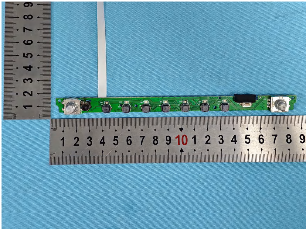
Photo 26 Internal photos of EUT
