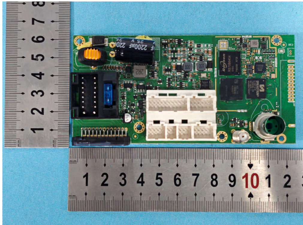
Photo 20 Internal photos of EUT Model: FG-9013 815-A
