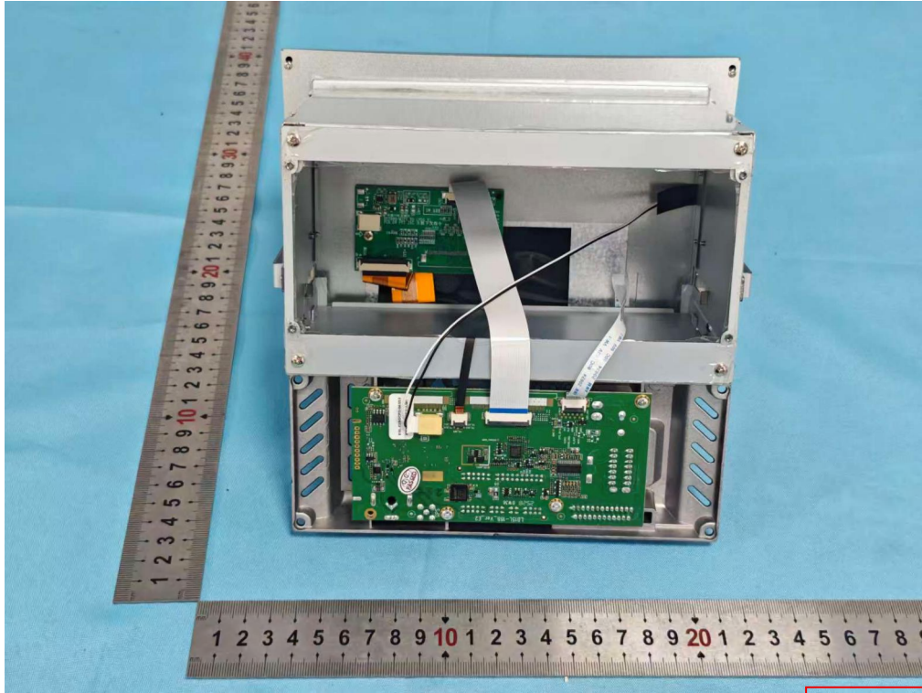
Photo 1 Internal photos of EUT Model: FG-9012 815-A
