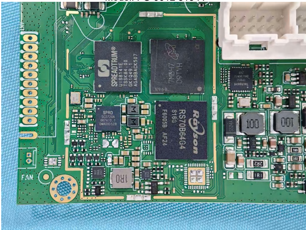
Photo 4 Internal photos of EUT Model: FG-9012 815-A
