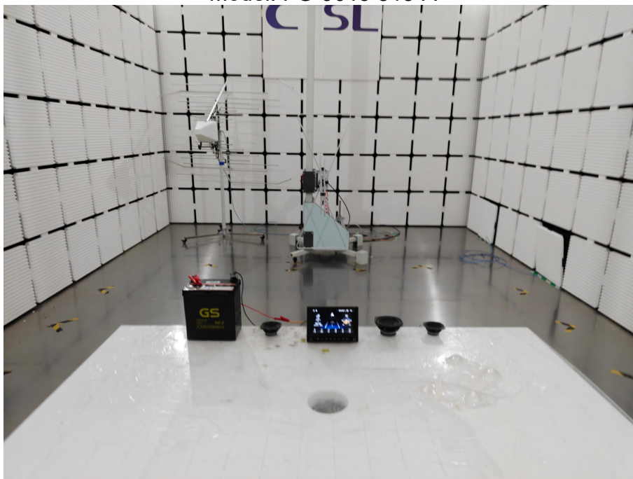
Photo 2 Test Setup Photos of Radiated Emission Test (30-1000MHz) Model: FG-9013 815-A
