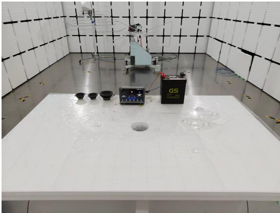
Photo 1 Test Setup Photos of Radiated Emission Test (30-1000MHz) Model: FG-9012 815-A
