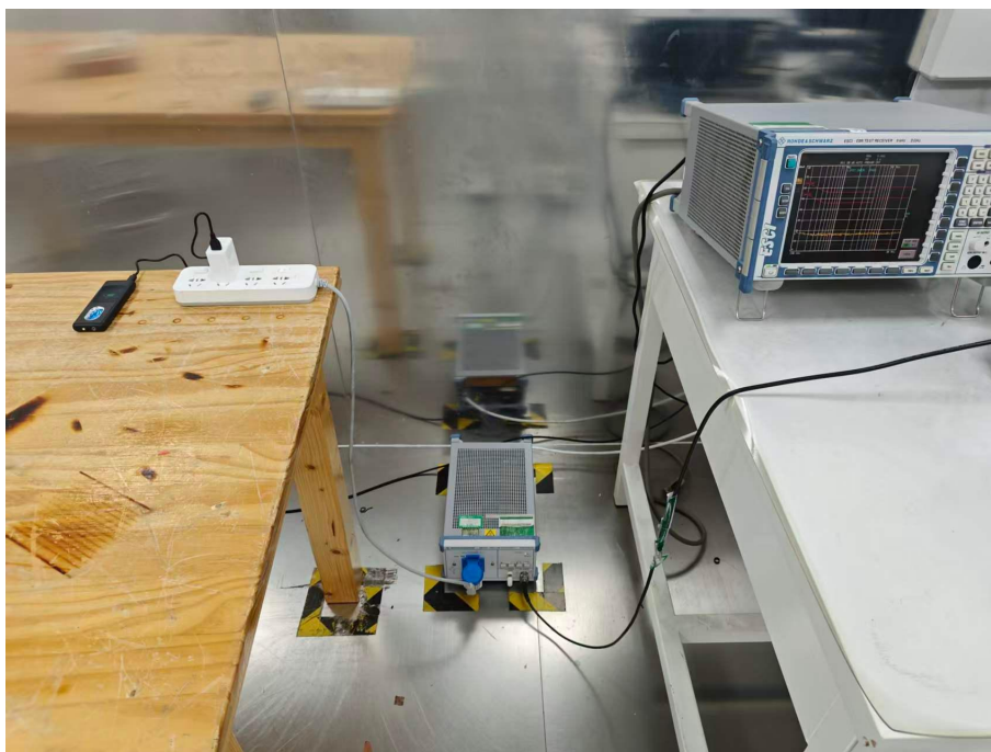
AC Port Conducted Emission
