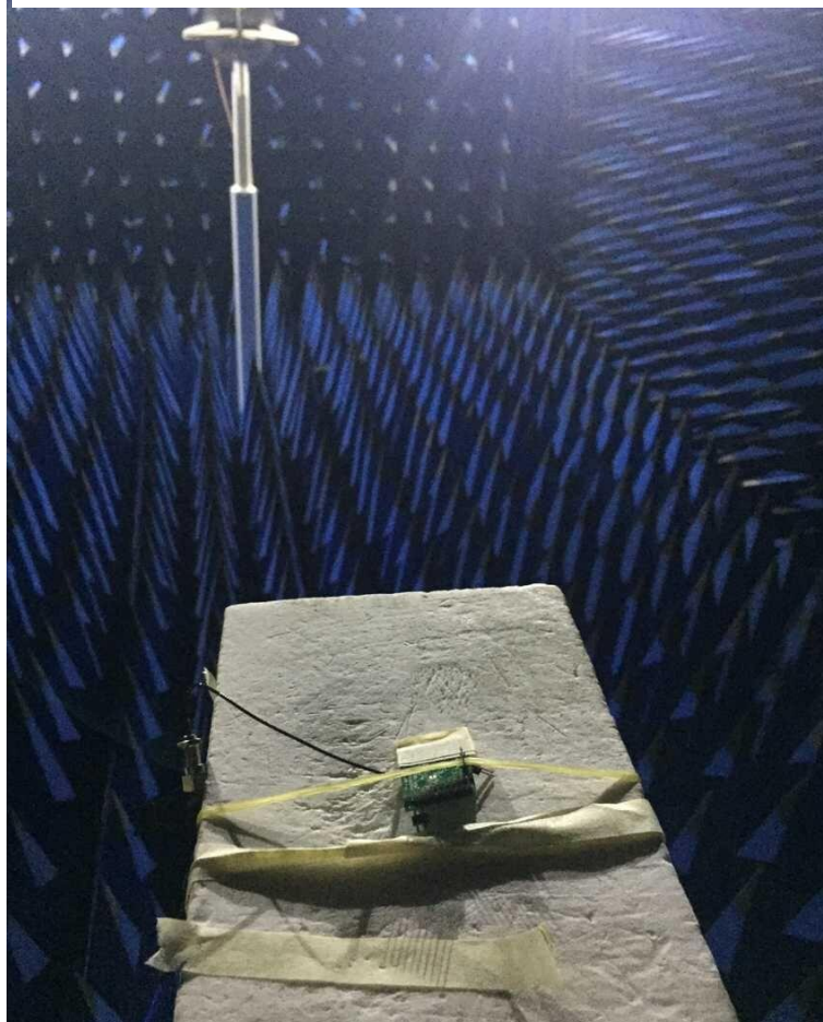
The Environment of Antenna Radiation Pattern
