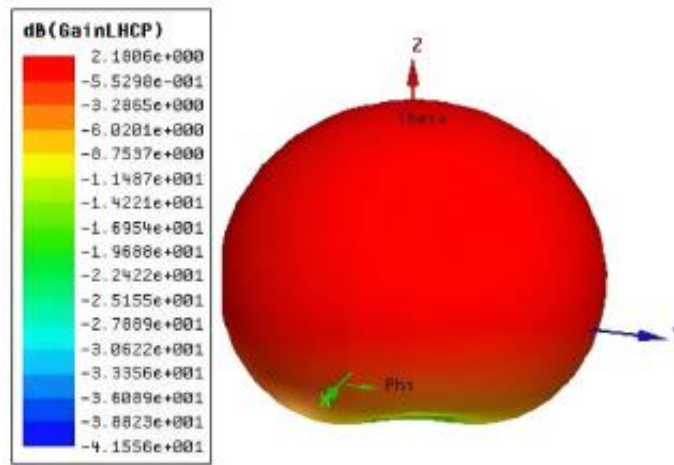
3D radiation pattern diagram
