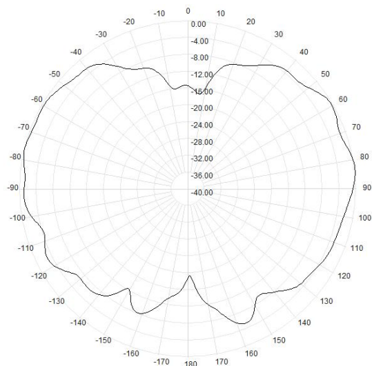
E(902MHz)
