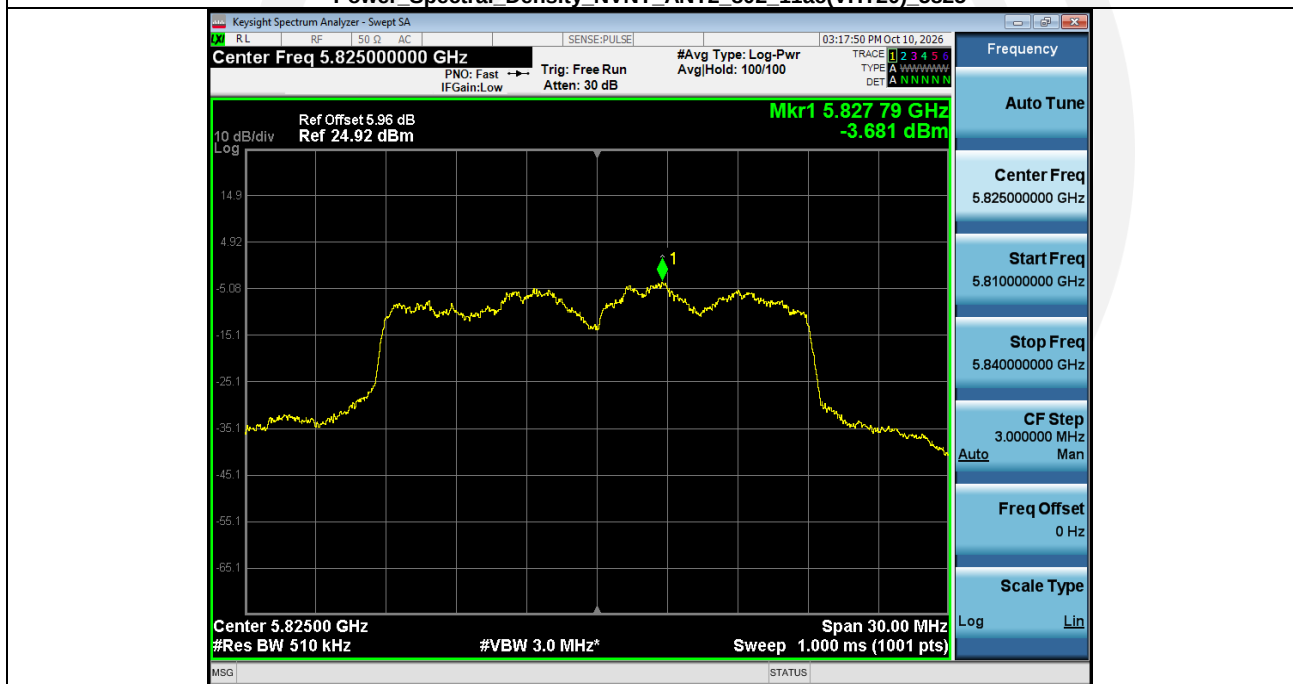
Power_Spectral_Density_NVNT_ANT2_802_11ac(VHT20)_5825
