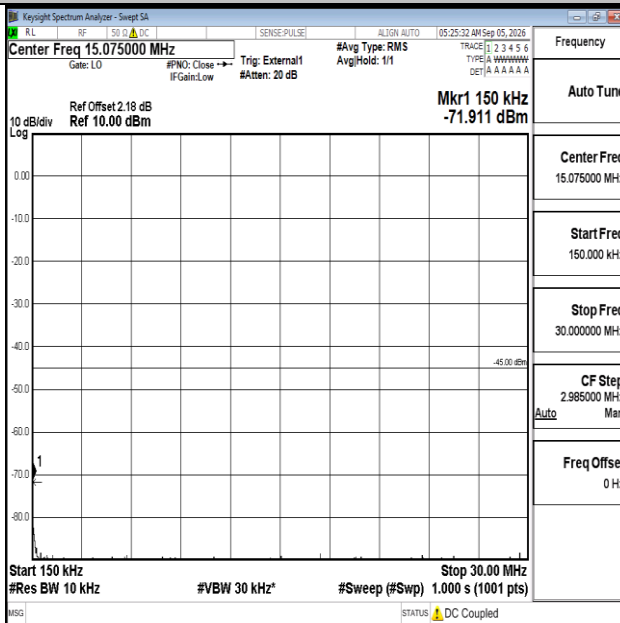
Band41-10MHz-QPSK-39700-1RB#0-0.15~30-PASS
