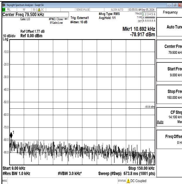
Band41-5MHz-QPSK-40620-25RB#0-0.009~0.15-PASS
