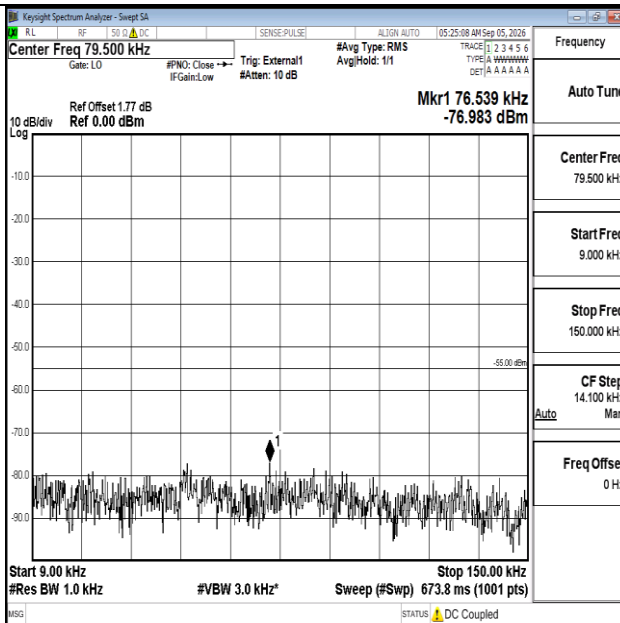
Band41-10MHz-QPSK-39700-1RB#0-0.009~0.15-PASS
