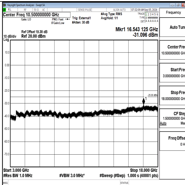
Band41-15MHz-QPSK-39725-75RB#0-3000~18000-PASS
