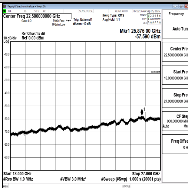
Band41-15MHz-QPSK-39725-75RB#0-18000~27000-PASS
