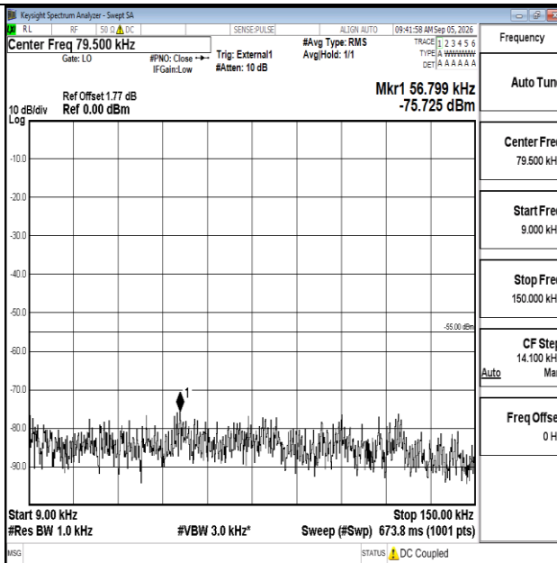
Band41-20MHz-QPSK-41490-1RB#0-0.009~0.15-PASS
