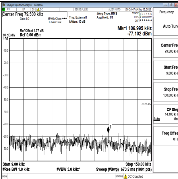
Band41-20MHz-QPSK-40620-1RB#0-0.009~0.15-PASS
