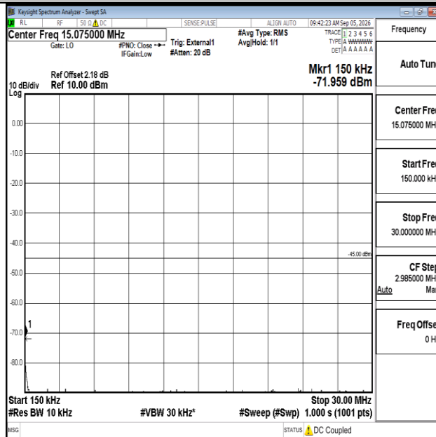
Band41-20MHz-QPSK-41490-1RB#0-0.15~30-PASS
