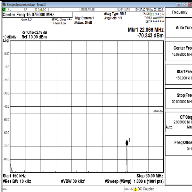
Band41-20MHz-QPSK-40620-1RB#0-0.15~30-PASS
