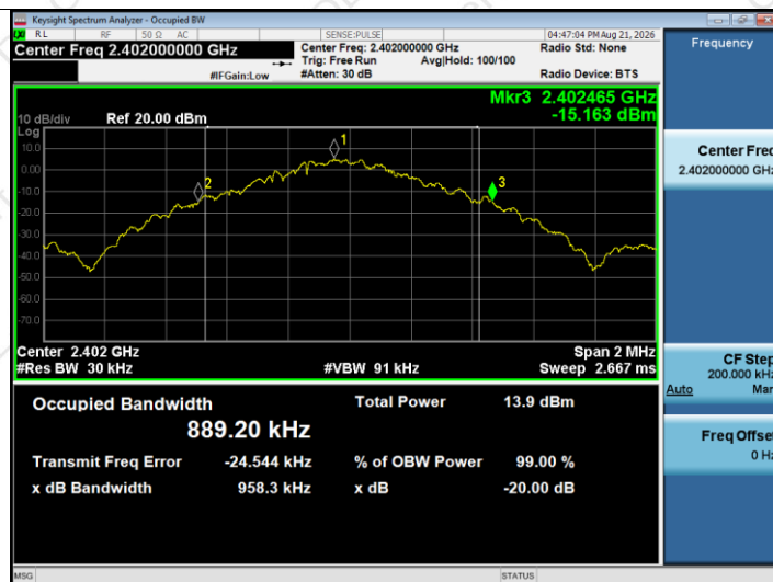
-20dB Bandwidth NVNT 1-DH5 2402MHz Ant1
