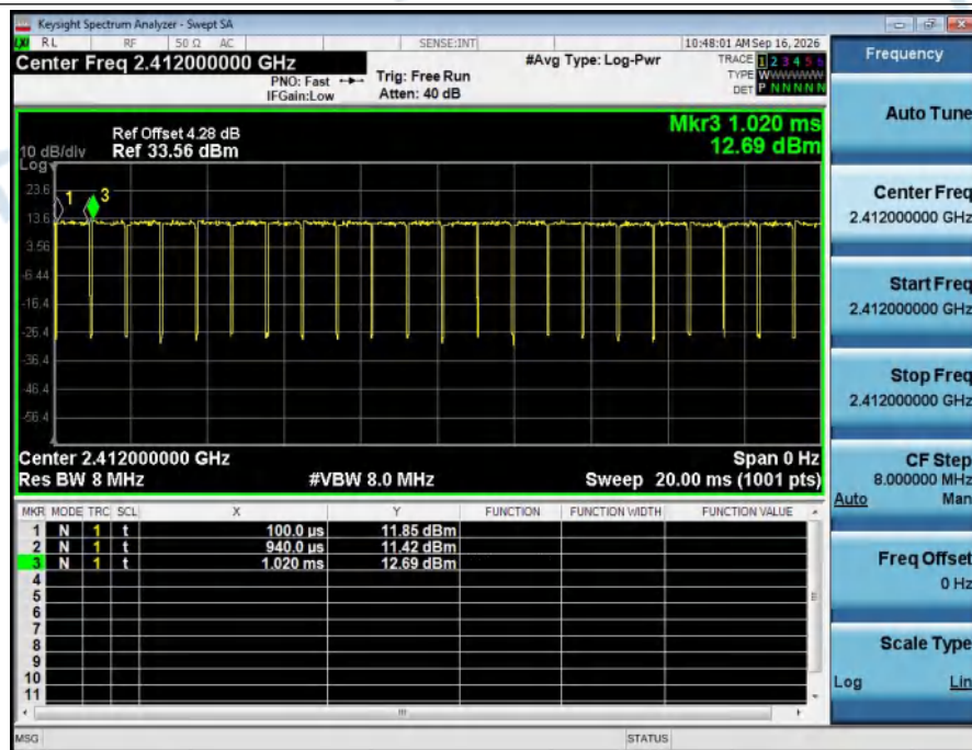
Duty_Cycle_NVNT_ANT1_802_11b_2412
