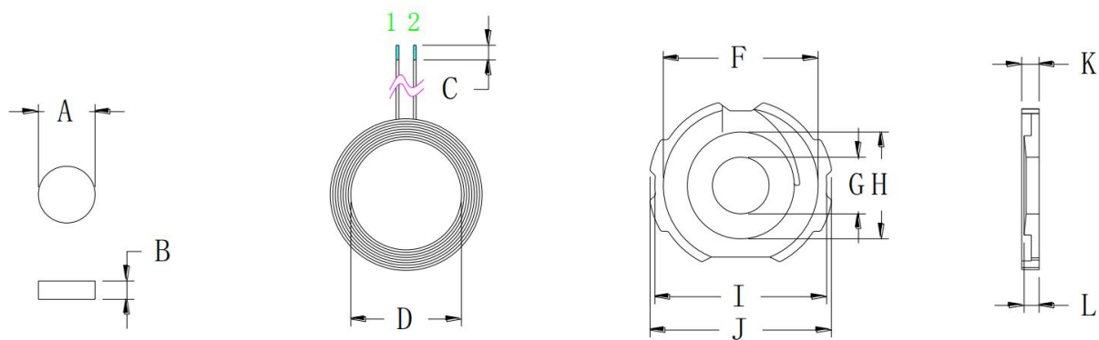
Plane Structure Diagram: Unit: mm
