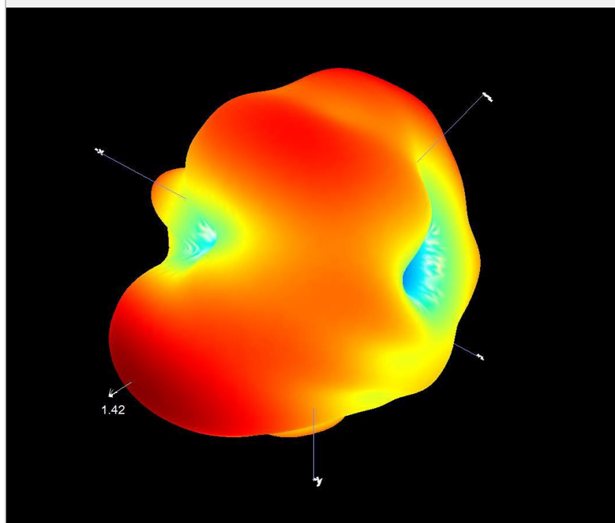
3D Pattern for 2400MHz
