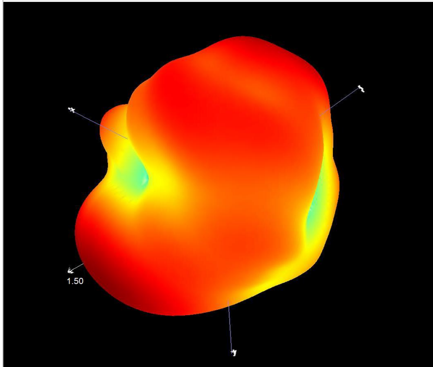
3D Pattern for 2450MHz
