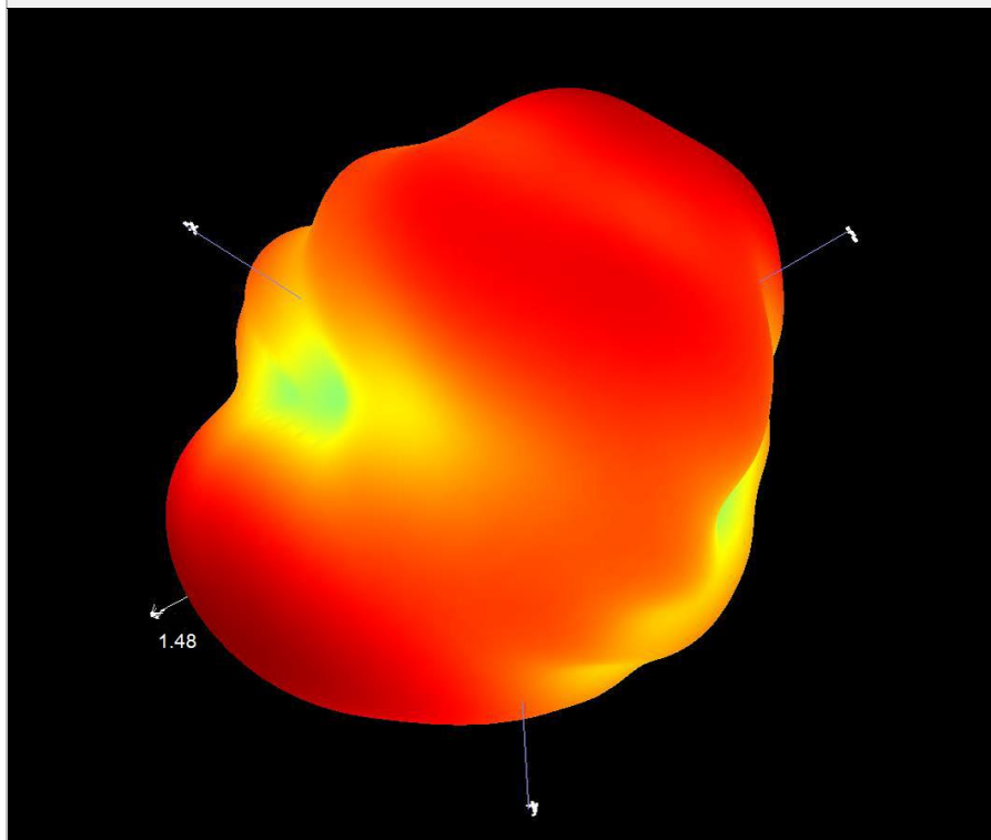
3D Pattern for 2500MHz
